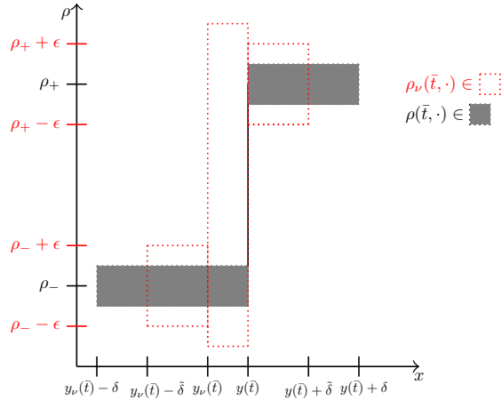
Figure 9: Illustration of Lemma A.3 in the case \rho_{\bar{u}}^* \leq \rho_- < \rho_+ and y_\nu(\bar{t}) < y(\bar{t}) . The approximate density \rho_\nu(\bar{t}, \cdot) in the space interval ]y_\nu(\bar{t}) - \tilde{\delta}, y(\bar{t}) + \tilde{\delta}[ belongs to the area surrounded by the red dotted lines, while \rho(\bar{t}, \cdot) in the interval ]y(\bar{t}) - \delta, y(\bar{t}) + \delta[ belongs to the grey shaded zone.
