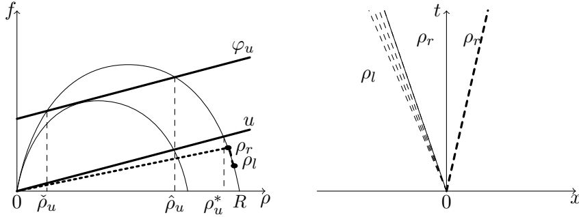
Figure 18: The Riemann problem. The situation of a rarefaction with speed less than u and f(\rho_r) < u\rho_r . In this case y(t) = uet , while the solution for \rho is composed by a classical rarefaction wave.
