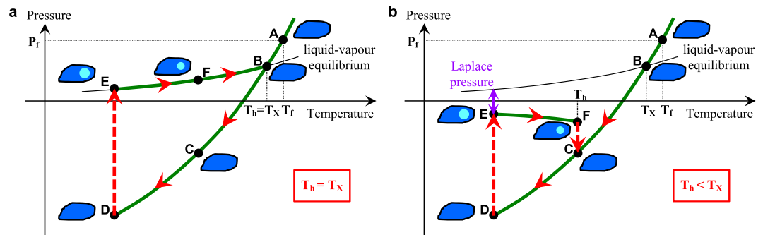
Figure 1. Schematic path followed by fluid inclusions (FIs). Note that the axis are not to scale. (a) Commonly assumed path. A monophasic FI is formed at a temperature T_f and pressure P_f (A). During cooling, the pressure of the liquid is reduced along an isochore (curve AB) and the liquid becomes metastable with respect to the vapour phase (curve BCD). This may lead to nucleation of a vapour bubble (transition from D to E), producing a biphasic FI (E). During heating, the FI follows the bulk liquid-vapour equilibrium (LVE) (curve EFB), the bubble shrinks, and eventually disappears at T_h = T_x (B). This assumption is valid for FIs with low fluid density and large volume. (b) Path modified by surface tension effects. Surface tension and the associated Laplace pressure lead to LVE at pressures below the bulk LVE (path EF) 33 . Eventually the bubble collapses (transition from F to C) at a temperature T_h , bringing back the FI on the isochore (curve ABCD). Surface tension thus causes T_h to be strictly less than T_x . This effect is relevant for FIs with high fluid density and small volume 33 . In contrast, warming the monophasic FI along the isochore and finding with Brillouin spectroscopy the crossing point B with the bulk LVE curve gives the correct T_x .
