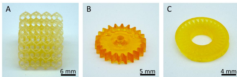
Fig. 4. Representative examples of thermoset parts fabricated from three different polymer classes: (A) Kelvin cell structure printed with polysiloxane SPR212, (B) cog wheel printed with polycarbosilane SMP10 and (C) turbine structure printed with polycarbosilazane Durazane1800.
