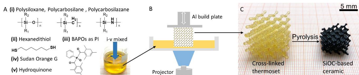
Fig. 2. Additive manufacturing of ceramics from preceramic polymers: schematic representation of thiol-ene click chemistry based stereolithography. (A) The preceramic photopolymerizable resin was prepared by mixing different preceramic polymers (polysiloxanes, polycarbosilane, polycarbosilazane) with 1,6-hexanedithiol dithiol along with phenylbis (2,4,6-trimethylbenzoyl) phosphine oxide (BAPOs) as photoinitiator (PI), Sudan Orange G as photoabsorber and hydroquinone as free radical scavenger (for more details, see Materials and Methods). (B) Photopolymerization of preceramic resins in a benchtop DLP printer utilizing a commercially available projector as a light source. (C) A representative printed cross-linked thermoset and the resultant glassy ceramic formed upon pyrolysis at 1100 ^{\circ}\text{C} under N 2 atmosphere.
