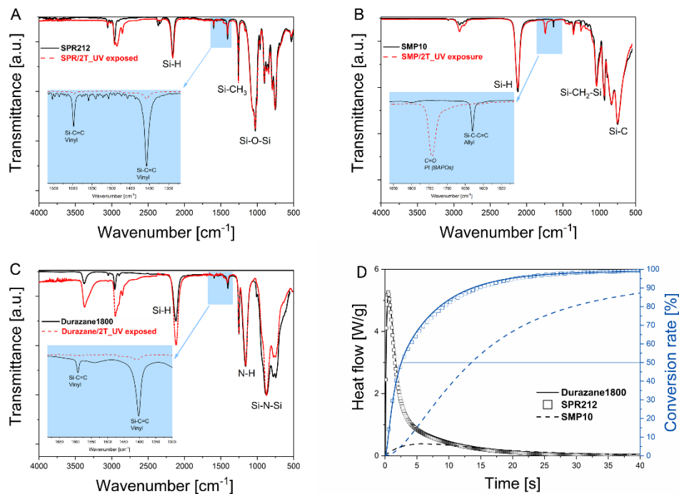
Fig. 3. (A-C) ATR-FTIR spectra of preceramic resins before (black) and after photoinduced curing (red): (A) with polysiloxane SPR212, (B) polycarbosilane SMP10 and (C) polycarbosilazane Durazane1800. The thiol-ene click polymerization is confirmed by the strong reduction of the absorption bands of the vinyl-groups. (D) In-situ differential scanning calorimetric characterization of preceramic resins exposed to light demonstrating that the preceramic resins are effectively cured within 15 secs, which makes them suitable for stereolithographic additive manufacturing: (black) the curing reaction heat and (blue) the conversion rate (the integral curve of heat flow after normalization)
