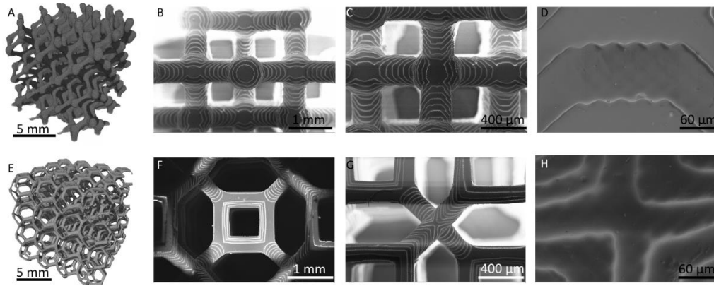
Fig. 8. Morphology and microstructure of additively manufactured SPR212-derived SiOC: (A and E) tomographic images of the diamond lattice (A) and Kelvin cell (E) structures. The delicate design is perfectly replicated without any detectable flaws. (B-D, F-H) Corresponding SEM images at higher magnification showing the step-like surfaces as well as the crack free struts.
