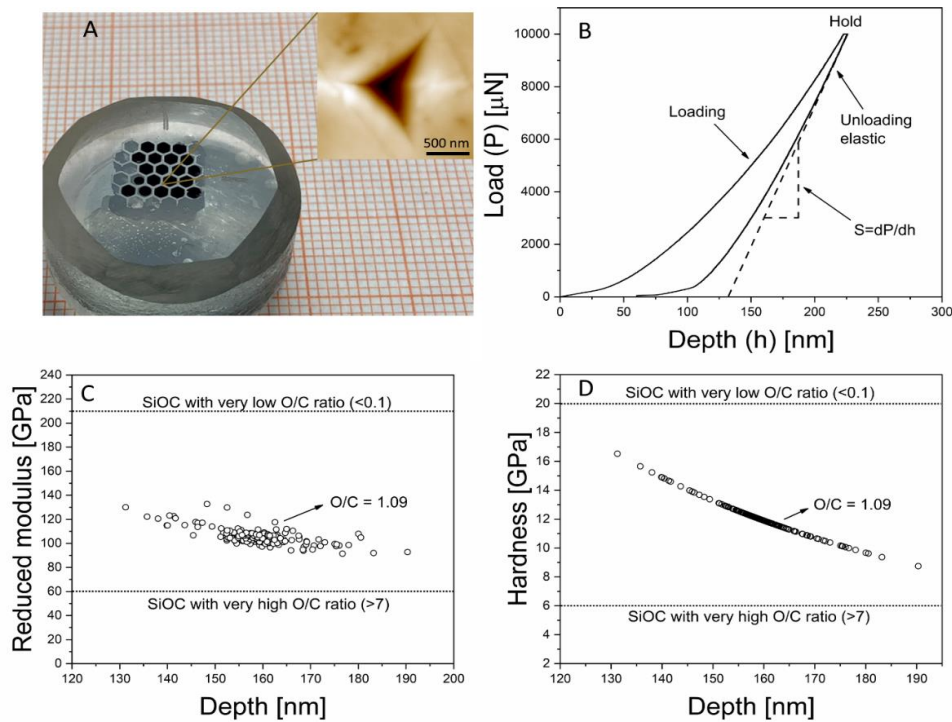
Fig. 9. Results of nanoindentation tests performed on 2D honeycombs of additively manufactured SPR212-derived SiOC. (A) A polished SiOC honeycomb imbedded in epoxy resin. Inset shows the AFM image of one indent. (B) Load-Hold-Unload curve of one indent. Elastic modulus is determined via the elastic unloading process. (C, D) Reduced modulus and hardness as a function of the penetration depth. 200 measurement results are shown here.
