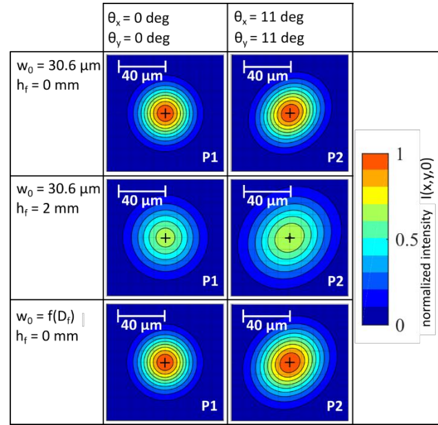
Figure 5. Energy distribution of the laser spot. The columns correspond to two positions of the laser spot P1 and P2. The rows correspond to three configurations (size of the laser spot fixed or depending on the focusing distance and defocusing equal to 0 or 2 mm).
