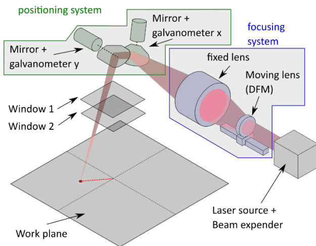
Figure 1. Opto-mechanical chain of an additive manufacturing machine by laser powder bed fusion. Post-objective focusing system.
