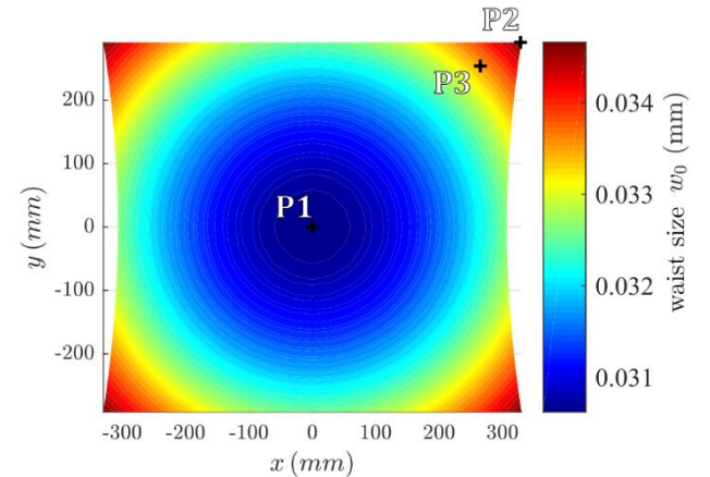
Figure 3. Variation of the waist size in the work plane.
