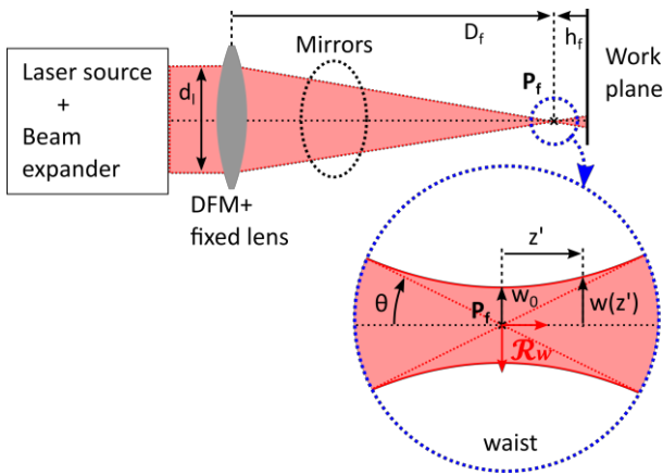
Figure 2. Parameterization and representation of the waist.
