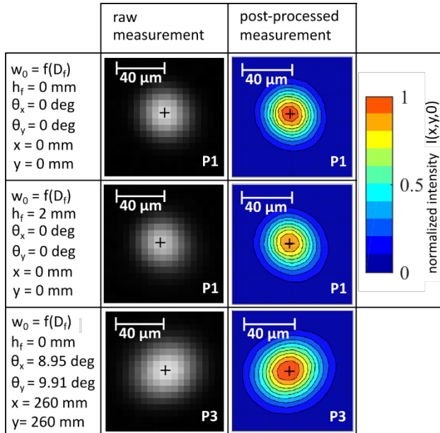
Figure 6. Experimental energy distribution of the laser spot. The three rows represent three different configurations. The left and right columns respectively represent the raw measurement and the post-processed measurement results.
