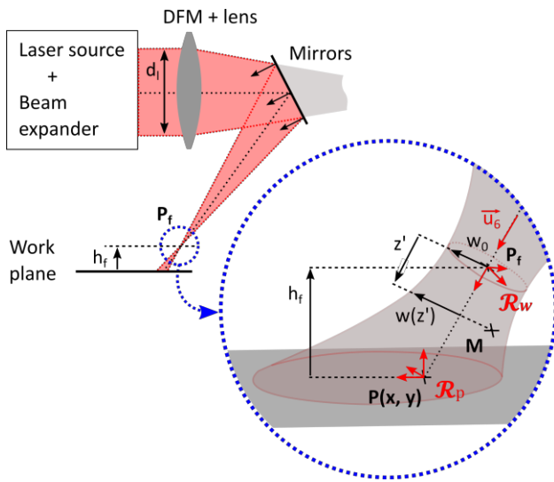
Figure 4. Intersection between the Gaussian laser beam and the work plane.
