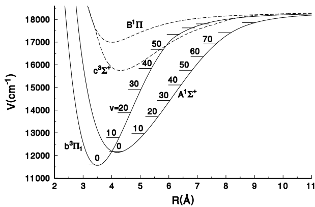
FIG. 7: NaK potentials for states that dissociate to \text{Na}(3^2S)+\text{K}(4^2P) . The c^3\Sigma^+ and B^1\Pi potentials (shown dashed) are not directly considered in the present Hamiltonian model. For the A^1\Sigma^+ and b^3\Pi_1 states, vibrational energies and numbers are indicated.
