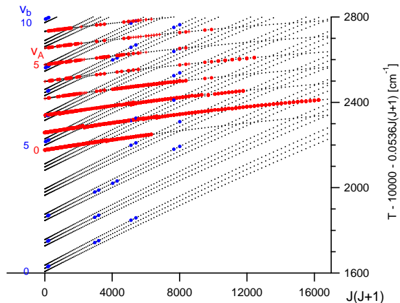
FIG. 9: (Color online) Rovibrational structure of mixed A-b states in two regions. The larger circles denote observed levels, the smaller circles are the results of multichannel calculations.
