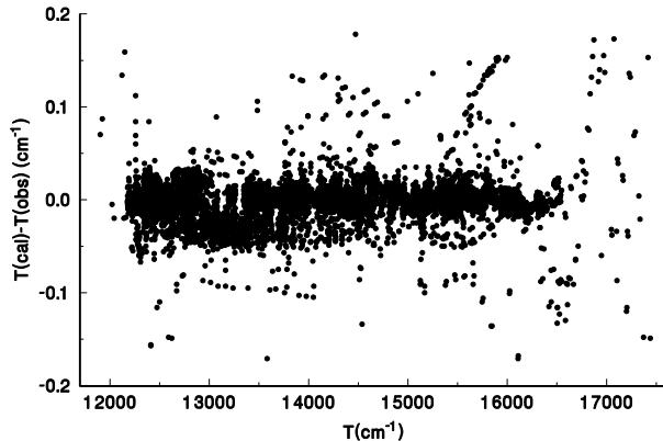
FIG. 6: Residuals from the fit to experimental observations of NaK transitions as deduced from term values of the X, B, C, d or D states and the transition wavenumbers. This plot does not indicate the experimental uncertainties, which are commonly 0.03 \text{ cm}^{-1} or less, but in some cases are more than 0.1 \text{ cm}^{-1} .
