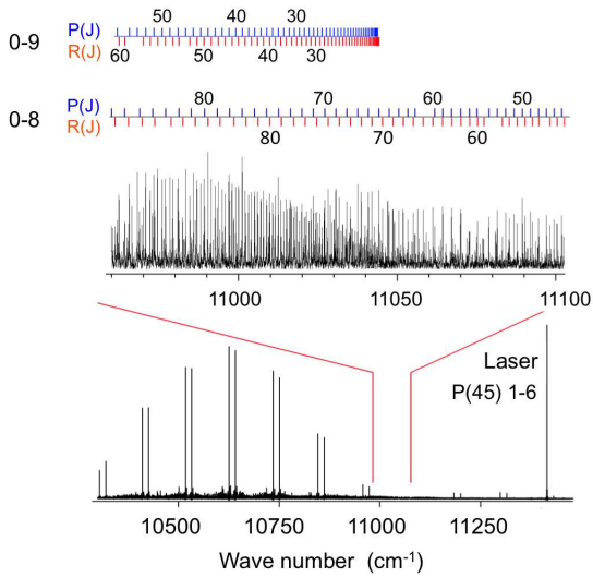
FIG. 3: (Color online) Fourier transform spectrum of laser-induced fluorescence following excitation of v = 1, J = 44 of the A state. The lower trace shows a typical sequence of P, R doublets. The upper section highlights the extensive vibrational relaxation, easily noticeable in the baseline of the spectrum.
