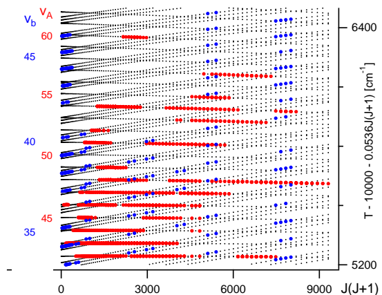
FIG. 12: (Color online) A continuation of the previous figure into higher
