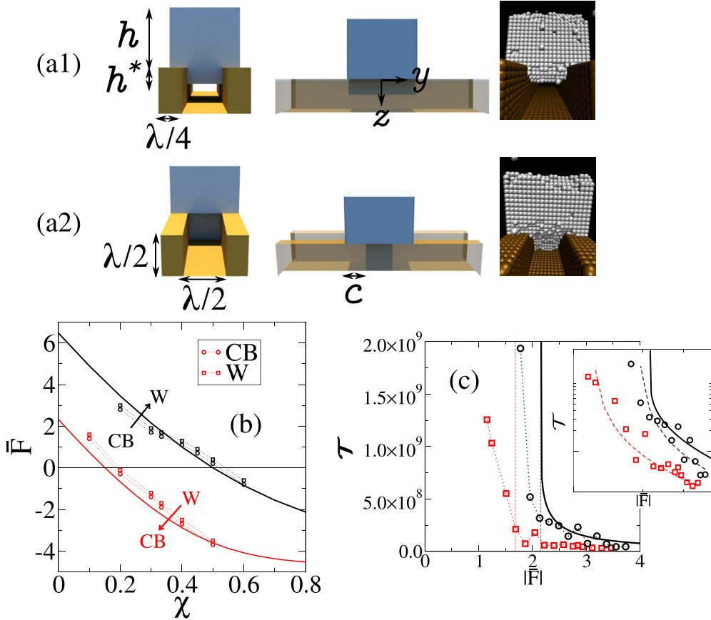
FIG. 2. (Color online) Migration-induced transitions. (a1, a2) Schematics of the intermediate configurations during the CB \rightarrow W and W \rightarrow CB transitions, and KMC snapshots. (b) Phase diagram in the presence of migration. The black solid line corresponds to the predicted transition from CB to W from Eq. (2). The prediction for the reverse transition from W to CB is the red solid line, corresponding to Eq. (5). The distance between the two lines indicates the presence of hysteresis. Symbols represent the final state in the KMC simulations: CB (circle) and W (square). The initial state is the W state for the upper curve ( W \rightarrow CB transition) and the CB state for the lower curve ( CB \rightarrow W transition). Other KMC parameters: \zeta = 0.2 , k_B T = 0.5J_1 , N = 20^3 , and \lambda = 20a . (c) Transition times \mathcal{T}_\downarrow (black) and \mathcal{T}_\uparrow (red), in units of 1/\nu_0 , as a function of |\bar{F}| . KMC simulation results: CB \rightarrow W (black circle) and W \rightarrow CB (red squares). The solid line is the analytical model for the CB \rightarrow W transition (described in Appendix A), with no fitting parameter. Other KMC parameters: \zeta = 0.2 , \chi = 0.3 , k_B T = 0.5J_1 , N = 20^3 , and \lambda = 20a . Inset: same data in log scale. The dashed lines correspond to \mathcal{T}_\downarrow = 0.7 \times 10^8 / (\bar{F} - 1.2) and \mathcal{T}_\uparrow = 10^8 / (\bar{F} - 1.9) .
