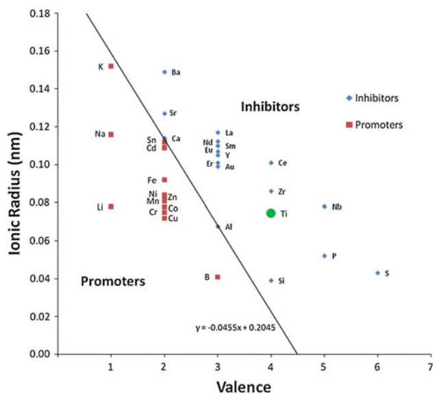
Fig. 11 Comprehensive valence/radius plot of anatase to rutile transformation, categorising inhibiting and promoting dopants, based on the published reports in Table 5
