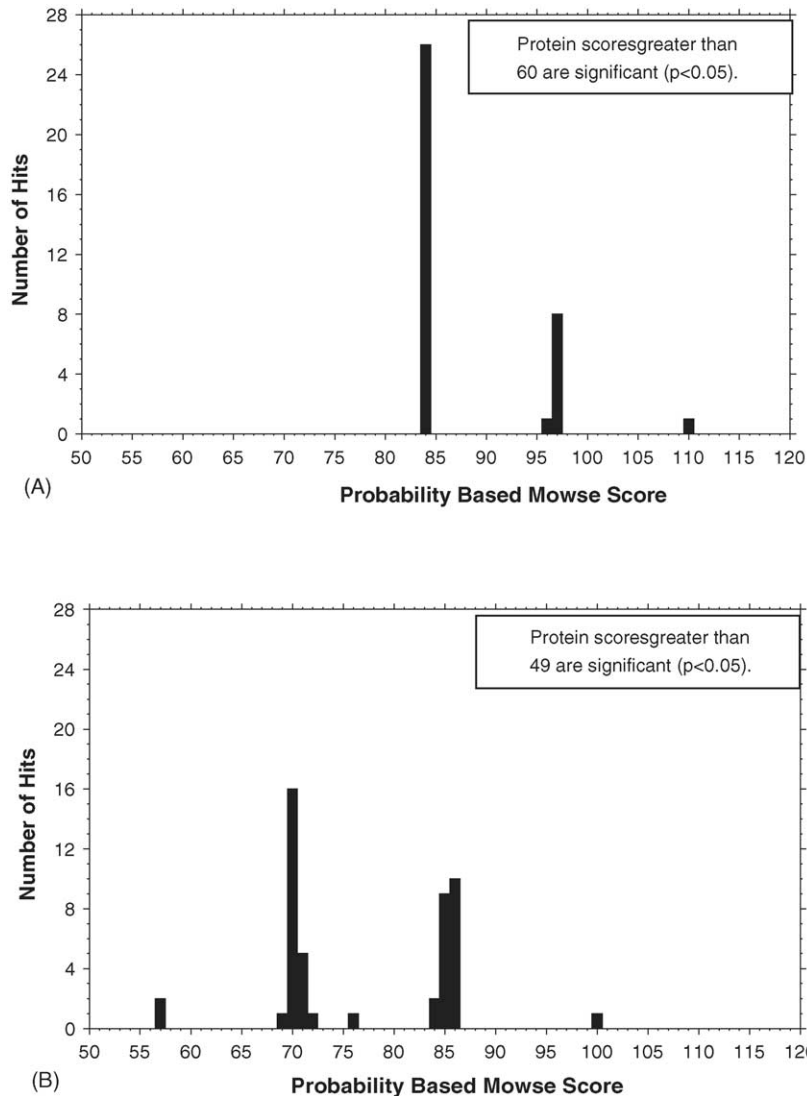
Fig. 3. Number of significant hits obtained with Mascot Server for Actin-2 of P. tricuspidatus (A) and S. tellinii (B).
