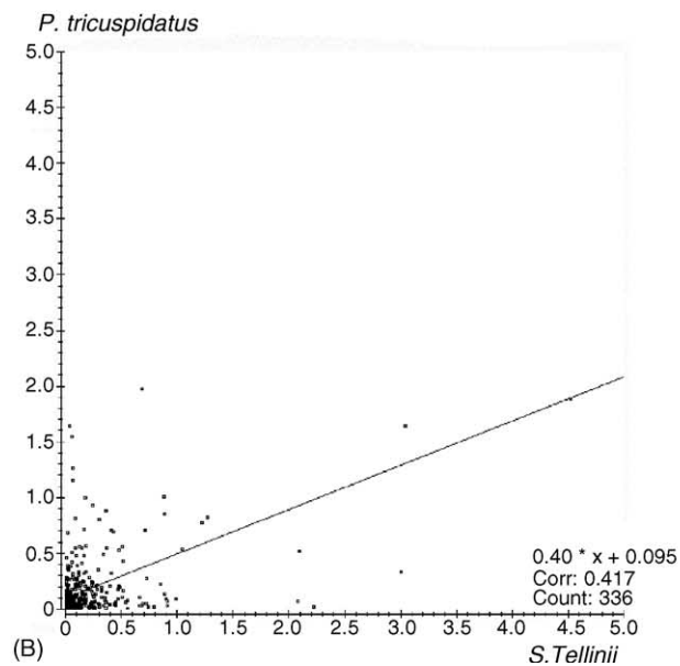
Fig. 2. (A) Two-dimensional synthetic gel issued from comparison between the protein patterns of Paragoridus tricuspidatus and Spinochordodes tellinii (a total of 928 spots). (○) Common protein spots ( n = 336 ); specific protein spots to P. tricuspidatus ( n = 353 ) (◐); specific protein spots to S. tellinii ( n = 239 ) (●); (B) Scatter plots on groups for the %volume.
