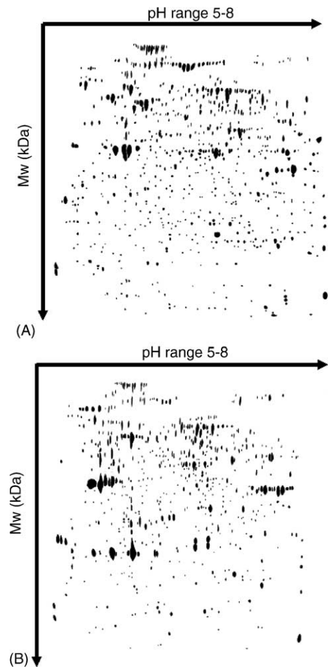
Fig. 1. Digitized two-dimensional gels of total soluble proteins extracted from two nematomorpha species: P. tricuspidatus (A) and S. tellinii (B).
