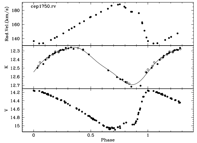
Fig. A.16. Light and radial velocity curves for the star OGLE-SMC-CEP1750.
