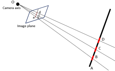
Fig. 3: Three collinear point framework for 3D pose estimation.
