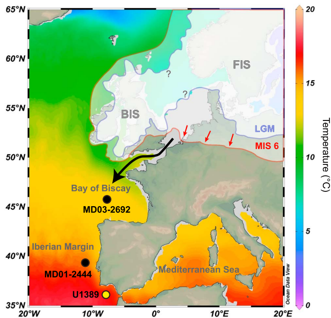
Figure 1. Map showing positions of Site U1389 and other locations along the European continental margin mentioned in the text, present-day mean annual sea-surface temperatures (50 m water depth), and maximum extent of European ice sheets during the Last Glacial Maximum and MIS 6 (Ehlers et al., 2011; Toucanne et al., 2015). FIS = Fennoscandian Ice sheet; BIS = British Ice sheet; dotted arrow = Fleuve Manche paleoriver. Sea surface temperatures are derived from the World Ocean Atlas 2013.
