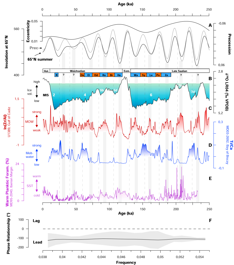
Figure 2. Terrestrial and marine proxy records for the Late Quaternary (0–250 kyr). (a) Eccentricity, precession, and summer (21 June) insolation curve for 65°N (Laskar et al., 2004). (b) Global benthic \delta^{18}\text{O} stack LR04 (Lisiecki & Raymo, 2005) as a measure of global ice volume. Marine Isotope Stages (MIS) follow Lisiecki and Raymo (2005). Corresponding continental glaciations and known ice advance and retreat phases are presented on top of panel b following the terminology for western and central Europe (Litt et al., 2007). Ze = Zeitz phase; Po = Pomßen interval; Le = Leipzig phase; Sy = Seyda interval; Wa = Warthe phase; He = Hering stadial; Br = Brörup interstadial; Re = Rederstall stadial; Od = Oderade interstadial; El = Ellund phase; Oe = Oerel stadial. (c) Zr/Al record from Site U1389 in the Gulf of Cadiz. Strong MOW phases are marked by grey bands. (d) Ti/Ca record from Site MD03-2692 in the Bay of Biscay (Toucanne et al., 2009). Peak Ti/Ca values are marked by black dashed lines. (e) Relative abundances of warm-water planktic foraminifera at Site MD95-2040 (see supporting information S5). (f) Phase relationship between the Zr/Al record from Site U1389 (reflecting MOW variability) and the Ti/Ca record from Site MD03-2692 (reflecting Fleuve Manche variability) for the precession band (frequency range = 0.039–0.053; 26–18 kyr). Mean phase value is indicated by black line; upper and lower 95% uncertainty levels are indicated by grey shaded area.
