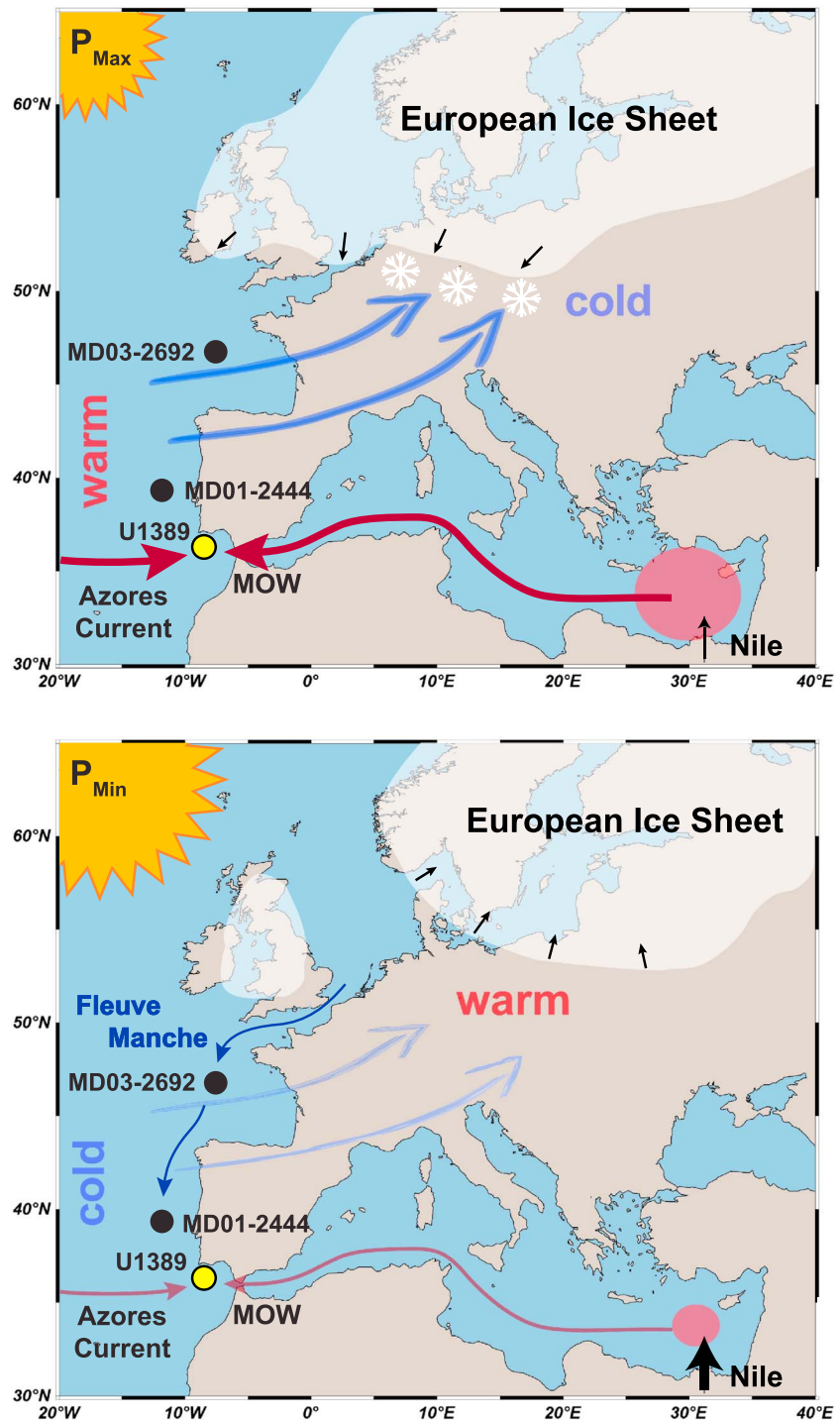
Figure 3. Schematic illustration of the insolation-driven modulation of European ice sheets. (a) During precession maxima (i.e., low insolation), aridity in NE Africa promotes MOW production, which enhances the strength of the Azores Current. Surface water warming off Iberia provides a source for moisture that is transported inland by deflected westerlies. Growth trajectories of the subsequent ice advances in continental Europe are directed toward the moisture source. (b) During precession minima (i.e., high insolation), the meltwater derived from the disintegration of the European ice-sheets feeds into the Fleuve Manche paleoriver and travels further south along the western European Margin. High summer insolation simultaneously strengthens the North African monsoon. This results in intensified freshwater discharge into the eastern Mediterranean Sea where it disrupts intermediate-water overturning and thereby reduces MOW production.
