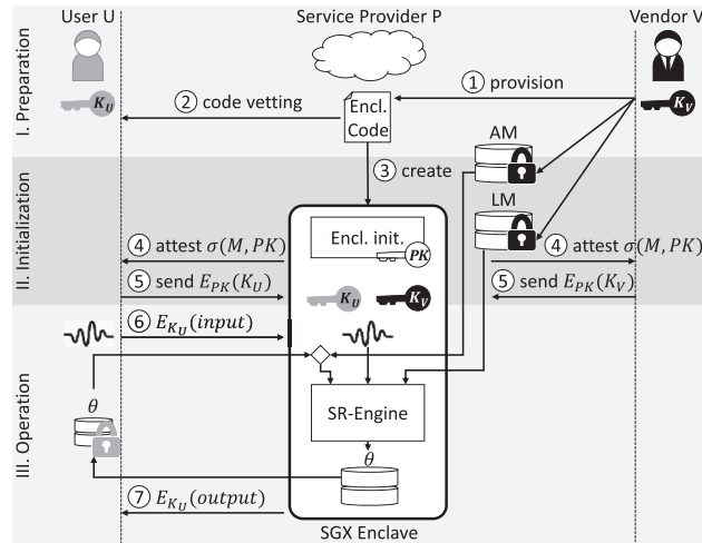
Fig. 7. VoiceGuard architecture using Intel SGX, taken from Brassler et al. (2018).
