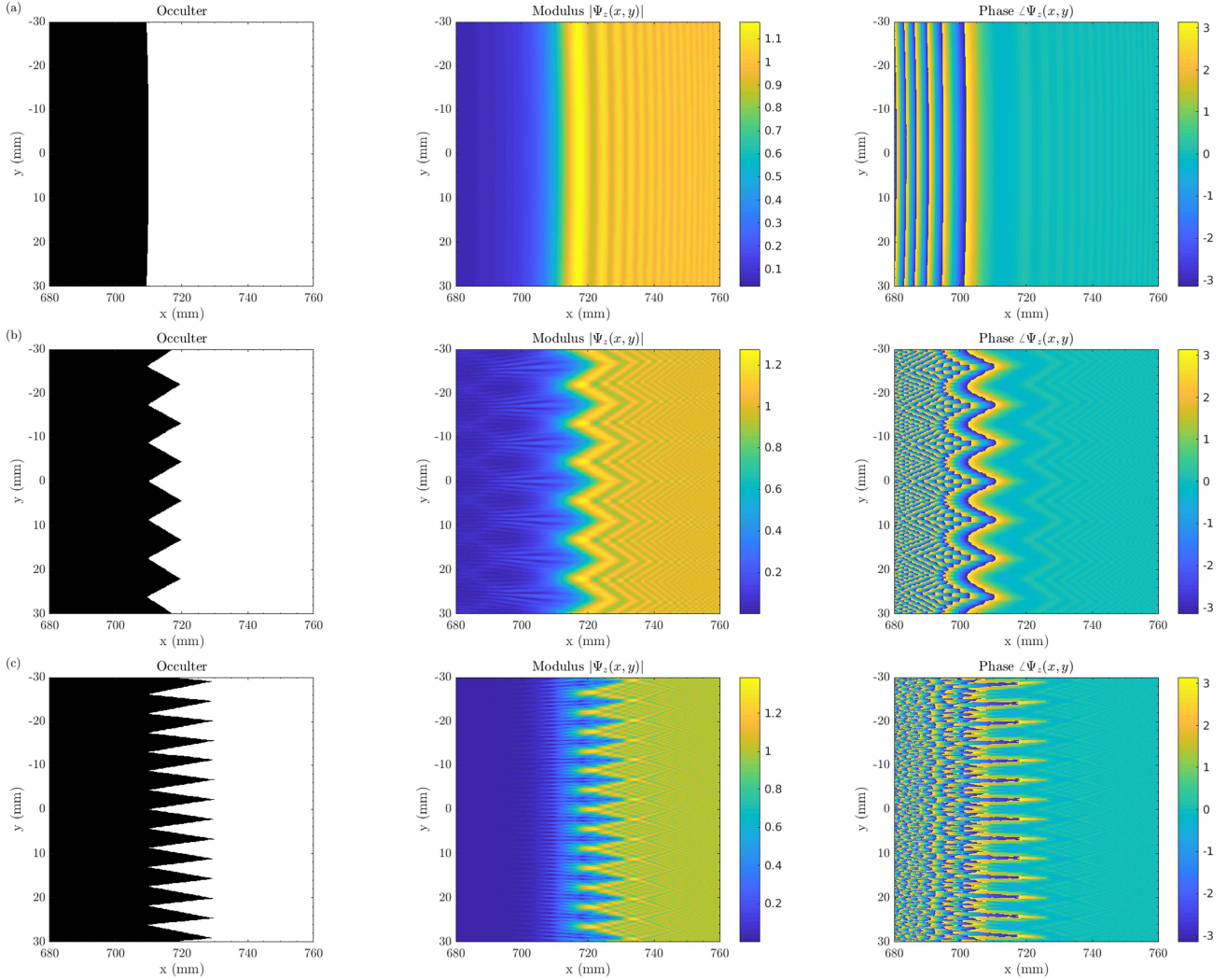
Fig. 5. 2D representation of the occulter, the modulus |\Psi_z(x, y)| , and the phase \angle\Psi_z(x, y) of the diffraction. The transition region between light and shadow is a rectangular zone of 80 mm \times 60 mm with a central position at 720 mm. From top to bottom: Panel a : circular sharp-edged occulter. Panel b : serrated occulter N_t = 512 and \Delta = 10 mm. Panel c : serrated occulter N_t = 1024 and \Delta = 20 mm.
