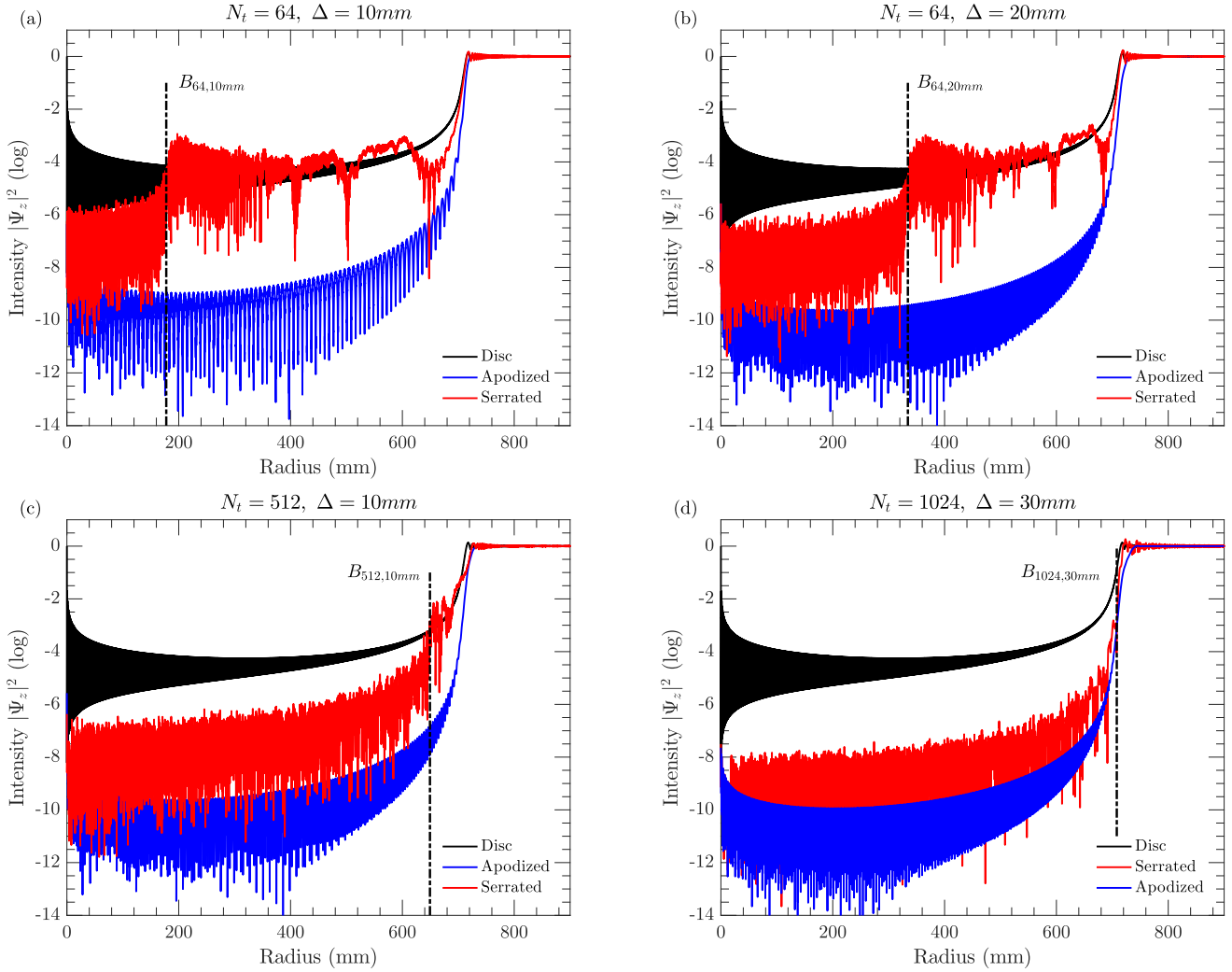
Fig. 6. Red: cuts of the diffraction intensity |\Psi_z(x, y)|^2 for several serrated occulters in logarithmic scale. The vertical lines shows corresponding Boivin radii B_{N_t, \Delta} . Black: sharp-edged disk. Blue: apodized disk. Panel a: N_t = 64 , \Delta = 10 mm. Panel b: N_t = 64 , \Delta = 20 mm. Panel c: N_t = 512 , \Delta = 10 mm. Panel d: N_t = 1024 , \Delta = 30 mm.
