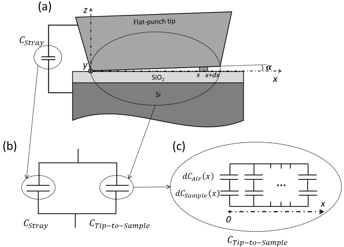
Figure 9: Capacitance modelling schematic.
