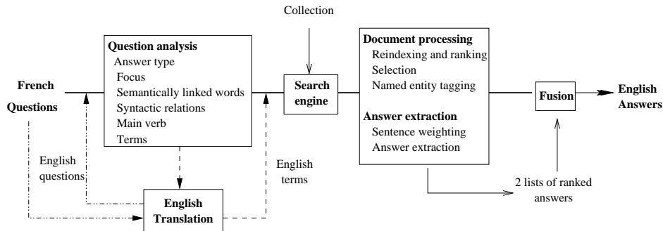
Fig. 1. MUSCLEF architecture
