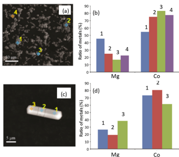
Figure 15: Illustrations of inhomogeneous metal mixing in MOF-74(Co/Mg), as revealed by SEM-EDX, between crystallites ((a) SEM image and (b) EDX point scans on the indicated positions in (a)) and within a crystallite ((c) SEM image and (d) EDX point
