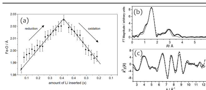
Figure 13: (a) In situ EXAFS observation of changes in the average Fe-O distance in the first coordination shell upon \text{Li}^+ insertion in MIL-53(Fe). Reprinted from ref. 56 with permission. Copyright 2009, Elsevier, (b) Comparison of the Fourier transform magnitude of the Fe K-edge EXAFS spectra for MIL-100(Sc(0.8)/Fe(0.2)) and (c) for MIL-100(Sc(0.5)/Fe(0.5)) containing also \alpha\text{-Fe}_2\text{O}_3 . Reprinted from ref. 55 with permission. Copyright 2014, John Wiley & Sons, Inc.
