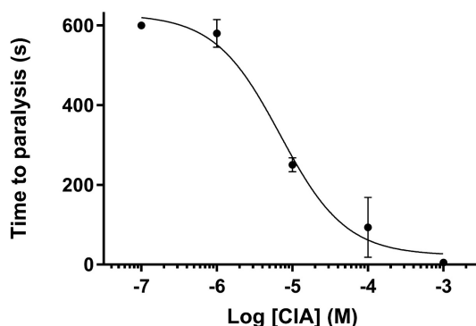
Figure 6. Paralytic effect of CIA on zebrafish. Paralysis induced by conotoxin \alpha -CIA shows a dose-dependent effect, with an IC_{50} of 6.88 \mu\text{M} .
