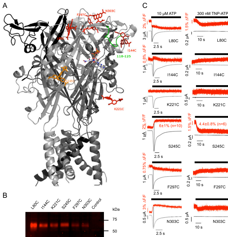
Fig. S6. Control experiments with P2X1 mutants in regions distant from the ligand binding domain (L80C, I144C, K221C, S245C, F297C, and N303C). (A) Position of these mutants in the P2X1 homology model. (B) Accessibility of the introduced cysteine residues as determined by labeling with TMRM and SDS/PAGE analysis. (C) Recordings from P2X1 mutants on application of 10 \mu M ATP and 300 nM TNP-ATP. Where applicable, averaged dF/F values are shown. The fluorescence changes in the L80C and S245C mutants suggest movements of these domains during ligand binding. EC 50 values (determined from three to four oocytes per mutant) ranged between 0.6 and 1.5 \mu M and thus, did not greatly differ from the WT P2X1 receptor.
