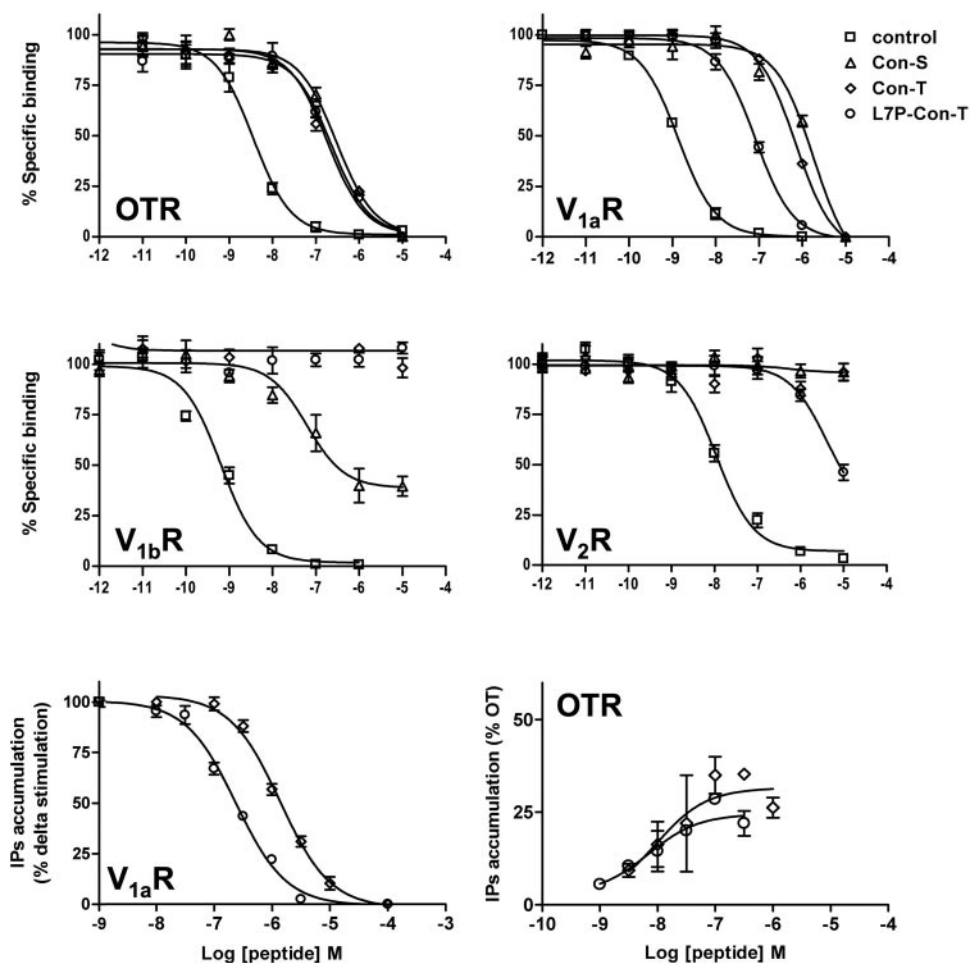
FIGURE 2. Binding and functional properties of Con-T and L7P-Con-T on human vasopressin and oxytocin receptors. A , Con-T (◇), Con-S (△), and L7P-Con-T (○) displacement of radioligands from OTR, V 1a R, V 1b R, and V 2 R receptors expressed in CHO cells. Control peptides were oxytocin (□) for the OTR and vasopressin (□) for all AVP receptors. B , functional properties of Con-T (◇) and L7P-Con-T (○) on human receptors. CHO cells stably transfected with V 1a R ( A ) or OTR ( B ) were grown in myo-[2- 3 H]inositol medium and IP accumulation measured and expressed as a percentage of levels stimulated by AVP and OT. Results are the mean ± S.E. of three separate experiments, each performed in triplicate.
