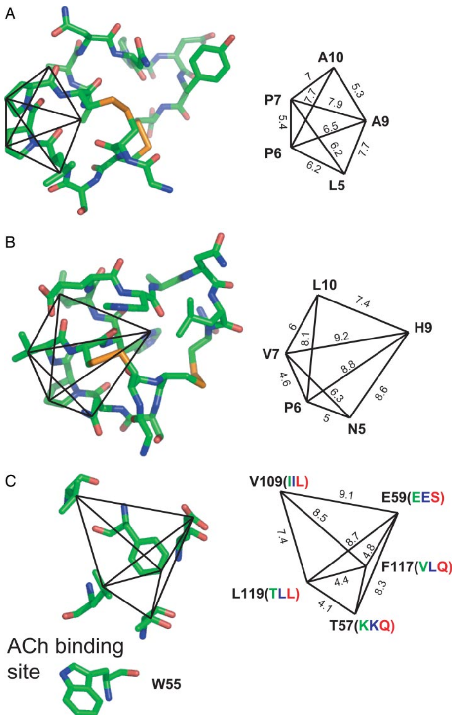
FIG. 9. \alpha -Conotoxin and \beta 2 subunit pharmacophores. PnIA (A) and MII (B) conotoxins are presented in their docked orientation in the cleft (C). The minimal pharmacophore shown is consistent with mutagenesis results and previous \alpha -conotoxin alanine scan data. Distances ( \text{\AA} ) between residues are measured from the last carbon of the side chain and reported on the vectors in the right-hand panels. Also shown are the equivalent residues for the \beta 3 (green), \beta 4 (blue), and (-) \alpha 7 (red) subunits. Note that Phe-117 is positioned under Glu-59.
