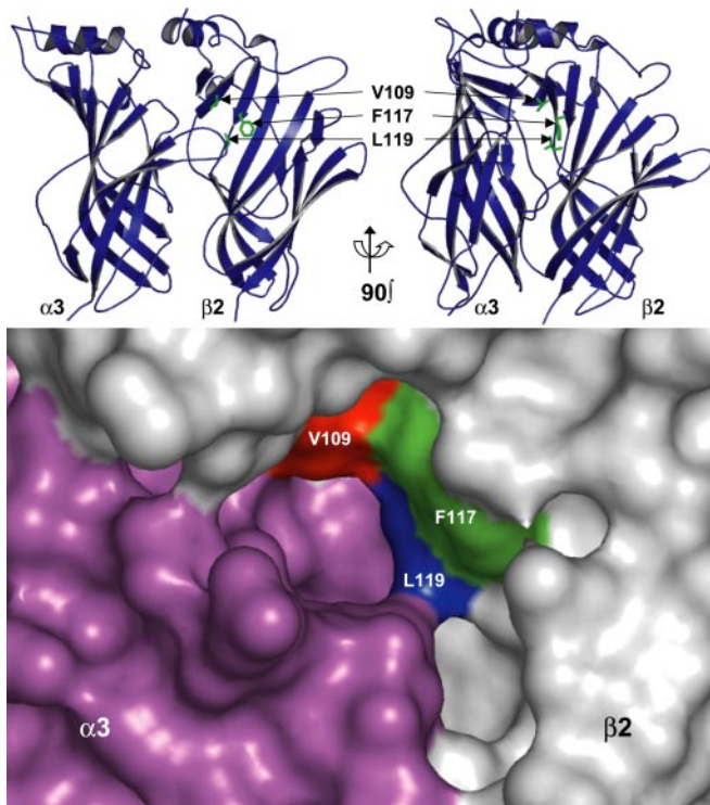
FIG. 1. Homology model of the \alpha 3\beta 2 nAChR showing the location of residues mutated in this study. A, ribbon representation of \alpha 3\beta 2 nAChR homology model with mutated residues in stick representation. B, enlarged view of the molecular surface of the \alpha 3/\beta 2 subunit interface showing the relative contribution of both \alpha 3 (purple) and \beta 2 (white) subunits to the cleft. Mutated residues are indicated.
