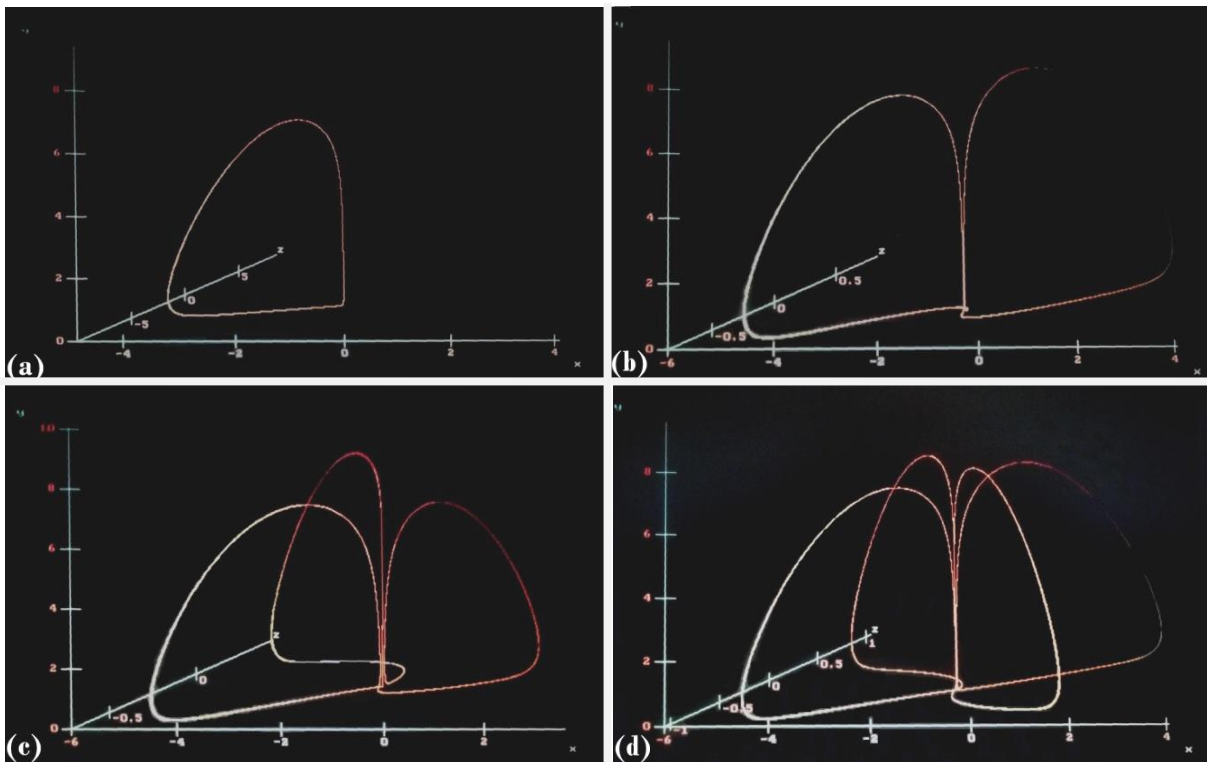
Fig. 4. A Sample of the Periodic Motions.
