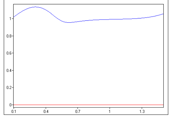
Fig.1. Spectrum of the largest Lyapunov exponent. Its value varies in the vicinity of the unit, which testifies to the chaoticity of the 3D model.
