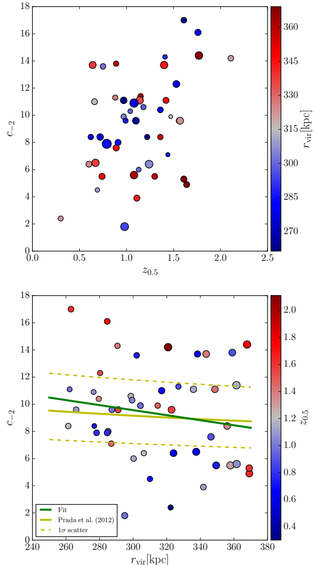
Figure 1. Overview of the host halo properties in the ELVIS suite. The top panel plots the halo concentration parameter c_{-2} against the formation redshift z_{0.5} , and color-codes for the virial radius r_{\text{vir}} . Larger symbol size indicate halos that host more extended sub-halo systems as measured via \Delta_{\text{r}}^{\text{subhalos}} . It is apparent that earlier-forming halos on average have higher concentration. The bottom panel compares the virial radius r_{\text{vir}} and concentration parameter c_{-2} . A linear fit (green line) indicates that more compact host halos (small r_{\text{vir}} ) tend to have slightly higher concentrations while larger halos have lower concentration, albeit with large scatter. This is in line with the expected mass-concentration relation, shown by converting M_{\text{vir}} to r_{\text{vir}} (yellow line from Prada et al. 2012). The dashed yellow lines indicate a 1\sigma scatter of 0.11 dex around the concentration relation (Macciò et al. 2008; Dutton & Macciò 2014). While the ELVIS halos follow the overall concentration relation well, the nine highest-concentration halos of the 48 host halos are on average offset by 2\sigma relative to the mean concentration relation.
