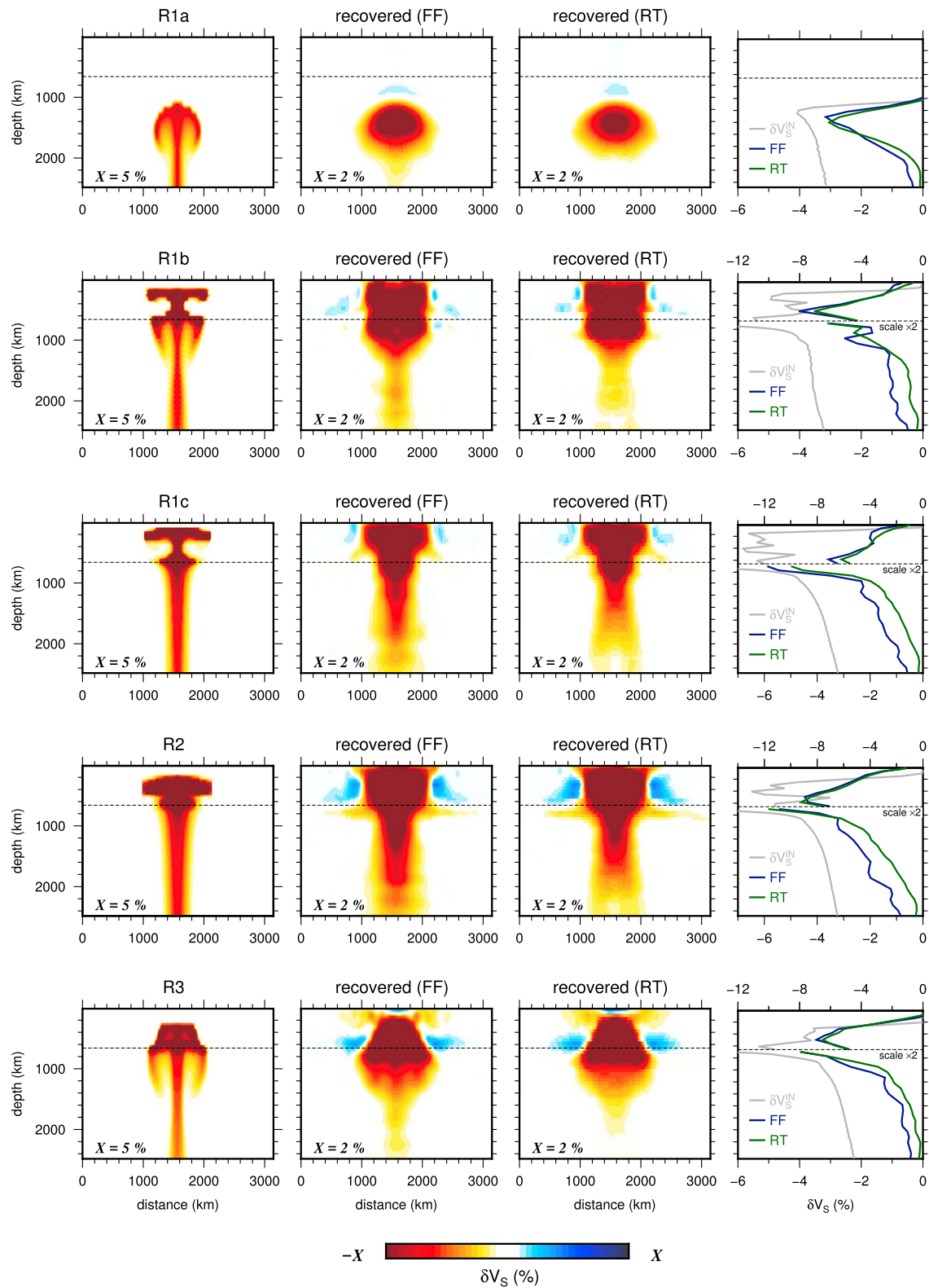
Figure 5. Shear velocity structures of the plumes R1, R2, and R3 obtained by inverting S wave delay times for network geometry A (Figure 4a) with L = 6,000 km, \Delta x = 100 km. The standard deviation of the traveltime uncertainty is \sigma = 0.1 s. (first column) The structures of the input plume models. (second and third columns) The resolved velocity structures using FF and RT. The dotted line is the 660 discontinuity. (fourth column) The resolved velocity structure along the plume axis for FF (in blue) and RT (in green), as well as the strength of the input structure \delta V_S^{IN} (in grey). The anomalies below the 660 are enlarged by a factor of 2 relative to the upper mantle for clarity.
