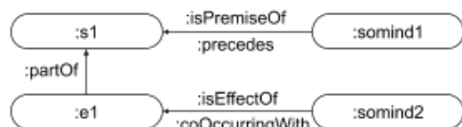
Fig. 12. A State_of_Mind :somind1 is a premise of a Session :s1 while :somind2 is an effect of an Experience :e1, part of :s1.
