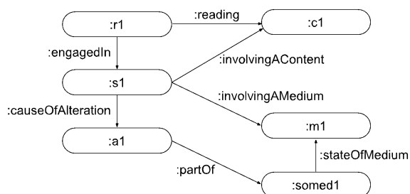
Fig. 11. A reader :r1 is engaged in a session :s1 , reading a content :c1 . The session :s1 involves the content :c1 and medium :m1 . Session :s1 is :causeOfAlteration :a1 , which is :partOf the State_of_Medium :somed1 , describing the state :stateOfMedium of the Medium :m1 . The relations :involvingAContent and :involvingAMedium are sub-properties of :involving . For readability, we omitted relations such as :m1 :providingAccessTo :c1 .
