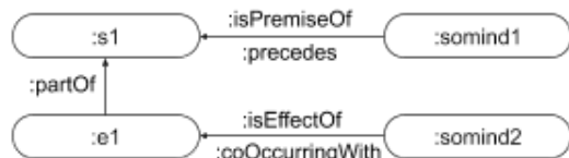
Fig. 11. A State_of_Mind :somid1 is premise of a Session :s1 while :somid2 is an effect of an Experience :e1, part of :s1.
