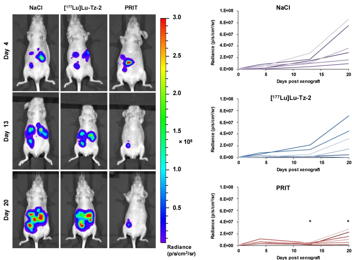
Figure 3: Longitudinal study of the PRIT of PC using [ ^{177}\text{Lu} ]Lu-Tz-2 and 35A7-TCO. After 9 days of tumor growth, mice bearing disseminated A431-CEA-Luc tumors were injected with either the treatment or the placebo. Control groups first received an i.v. injection of NaCl followed 24 h later by an i.p. injection of either NaCl or 40 MBq of [ ^{177}\text{Lu} ]Lu-Tz-2. The PRIT group first received an i.v. injection of 50 \mu\text{g} of 35A7-TCO, followed 24 h later by an i.p. injection of 40 MBq of [ ^{177}\text{Lu} ]Lu-Tz-2. Left: In vivo bioluminescence imaging at different time points post-treatment. Right: In vivo tumor growth was monitored and quantified from 4 to 20 days post-treatment using bioluminescence imaging. * p < 0.05 : day 13 and day 20 of PRIT group vs day 13 and 20 of NaCl and [ ^{177}\text{Lu} ]Lu-Tz-2 control groups (one-way ANOVA test).
