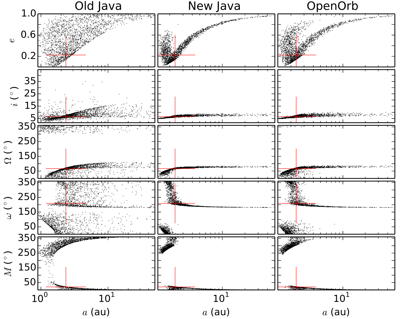
Fig. A.3. Same as Fig. 4 but for asteroid (420834) 2013 JX 10 with six transits.
