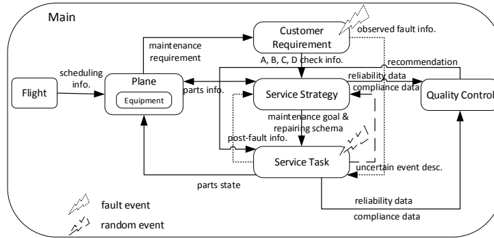
Figure 4: The architecture model of the agent-based simulation system
