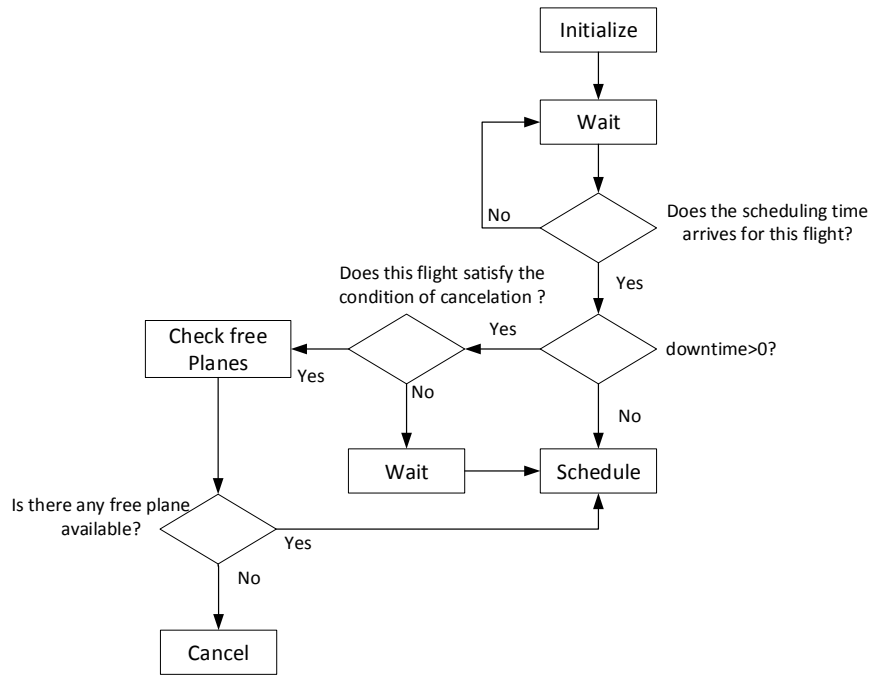
Figure 5: The flowchart of flight scheduling strategy
