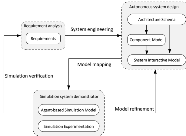
Figure 1: Autonomous system framework for aircraft maintenance
