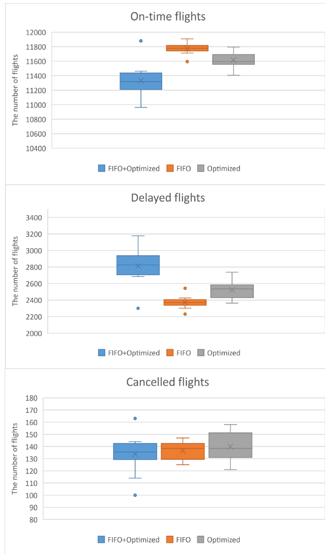
Figure 10: The impacts of maintenance sequence strategies on service level
