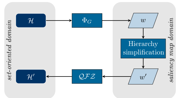
Fig. 1. A flowchart of the proposed method for removing non-significant regions from a given hierarchy \mathcal{H} and obtaining a new hierarchy \mathcal{H}' .
