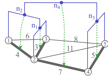
Fig. 3. Given a weighted graph, its minimum spanning tree T (whose edges are thick and gray) is represented by the binary partition tree by altitude ordering B (in blue). Each leaf node corresponds to a vertex of T while each non-leaf node n_i of B corresponds to an edge of T ; the correspondences are depicted in green arrows.
