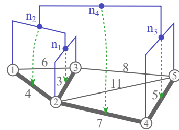
Figure 3: Given a weighted graph, its minimum spanning tree T (whose edges are thick and gray) is represented by the binary partition tree by altitude ordering B (in blue). Each leaf node corresponds to a vertex of T while each non-leaf node n_i of B corresponds to an edge of T ; the correspondences are depicted in green arrows.
