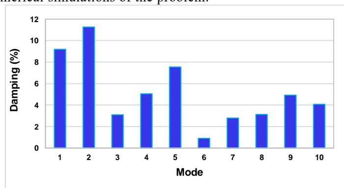
Figure 8 – Experimental modal damping of the double-glazing
