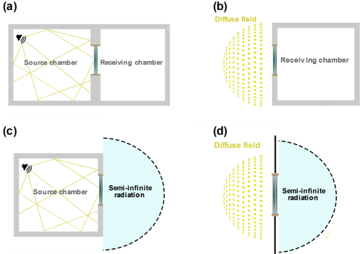
Figure 10 – Different configurations considered for problem resolution
