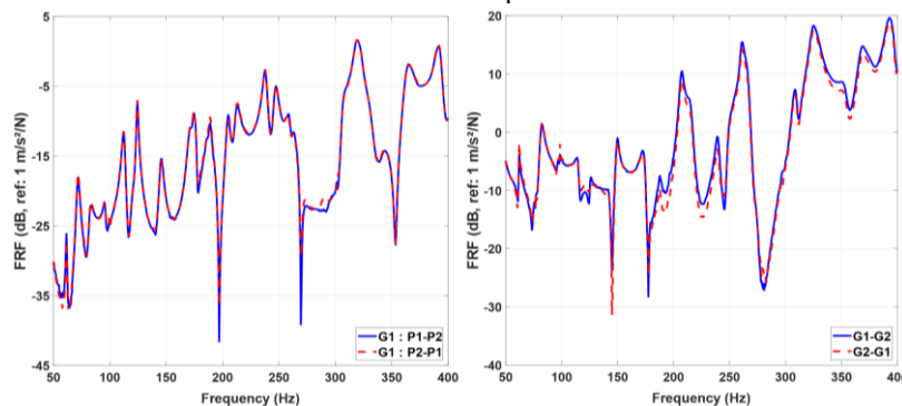
Figure 6 – Verification of the reciprocity
