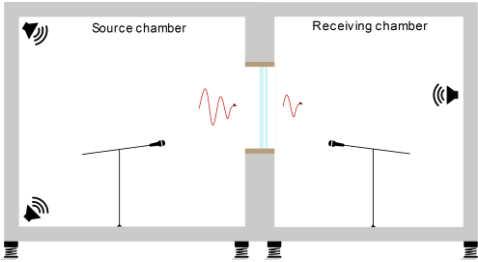
Figure 9 – Experimental set-up of acoustic experimental test
