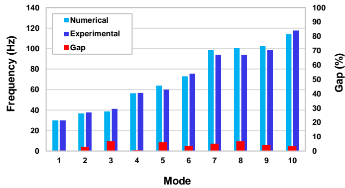
Figure 7 – Comparison of the first ten experimental and numerical eigenfrequencies of the double-glazing
