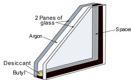
Figure 3 – Details of the double-glazing
