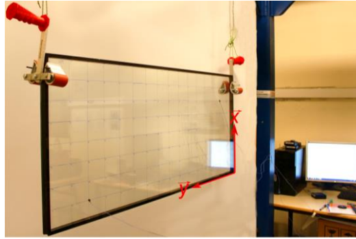
Figure 5 – Suspended double-glazing
