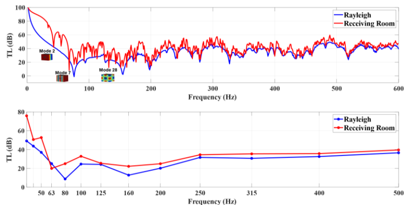
Figure 11 – Comparison of the TL between the two configurations in the narrow and 1/3 octave band
