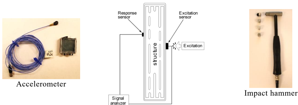
Figure 4 – The device of modal analysis
