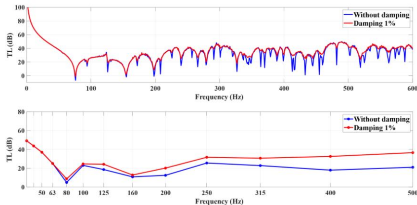
Figure 12 – Effect of the damping in the TL of the double-glazing (configuration d)
