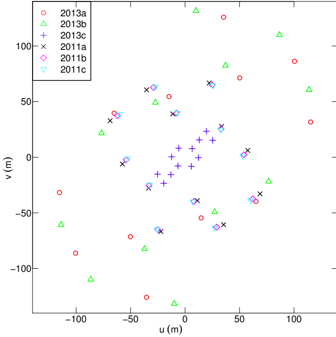
Fig. 1. (u, v) plane coverage of our interferometric observations.
