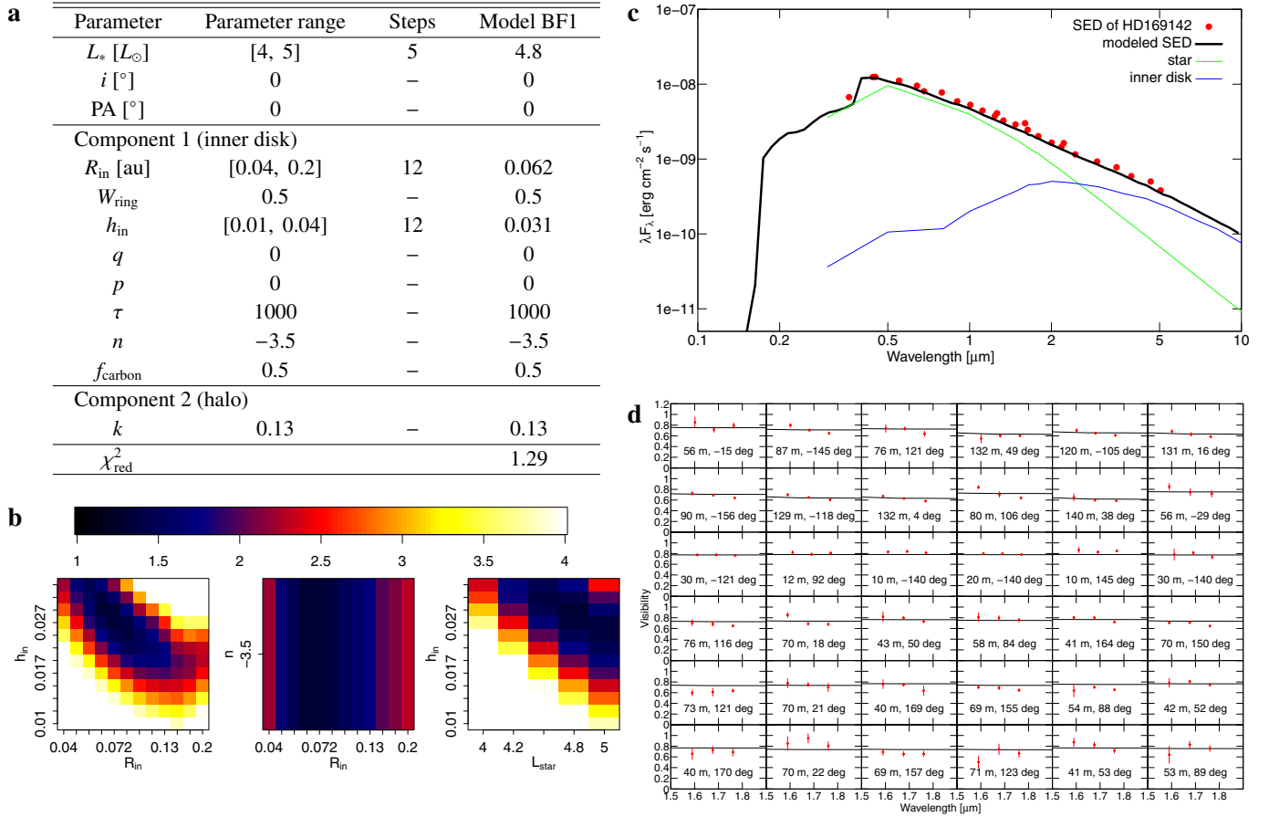
Fig. 5. As Fig. 4, but for model run BF, compared with the data set. Model BF1 is the model with minimum \chi^2_{\text{red}} .
