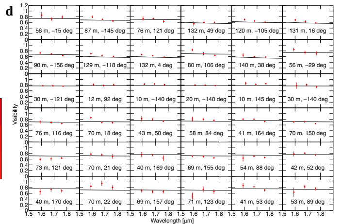
Fig. A.1. As Fig. 4, but for model run A, compared with the data set. Model A1 is the model with minimum \chi_{\text{red}}^2 .
