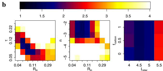
Fig. A.1. As Fig. 4, but for model run A, compared with the data set. Model A1 is the model with minimum \chi_{\text{red}}^2 .
