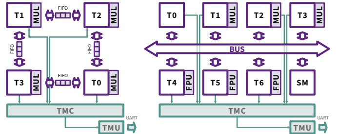
Fig. 5. We use a homogeneous platform with 4 peer-to-peer connected tiles (left) and a heterogeneous one with 7 tiles (right) connected via a shared interconnect. Some tiles have Floating Point Units (FPU) or hardware multiplier (MUL). In green the measurement infrastructure is shown with the Time Measurement Controller (TMC) that merges all control signals from the tiles to trigger the Time Measurement Unit (TMU).
