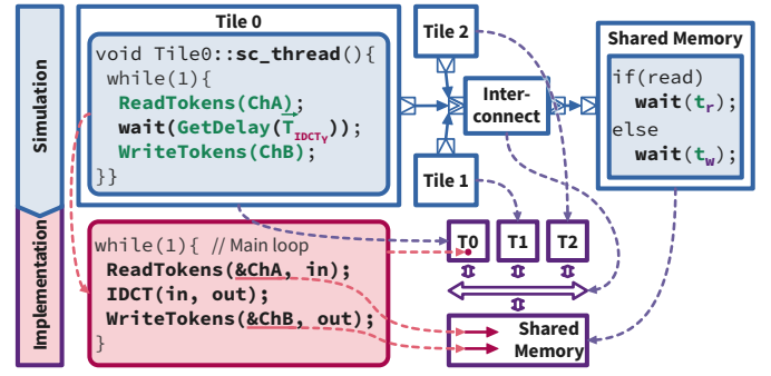
Fig. 3. Overview of our SystemC model with 3 tiles and how it is related to the later implementation of the simulated system. Tile 0 is presented in detail, with one actor (IDCT Y ) mapped on it.
