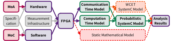
Fig. 1. Overview of our workflow. Hardware and Software gets designed following specific models. Then one instance of the system on an FPGA gets characterized. The resulting model can then be analyzed for real time properties (green). For evaluation we also create a static mathematical model shown with dashed red lines. And in dashed orange lines, only observed WCET gets considered.
