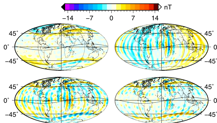
Fig. 3 Difference at Earth's mean radius between V-ASM and Z-ASM models at epoch 2014.3 and for the full expansion. From top left to bottom right, B_X , B_Y , B_Z , and B , respectively. Thin lines indicate magnetic equator and 50° magnetic quasi-dipole latitudes
