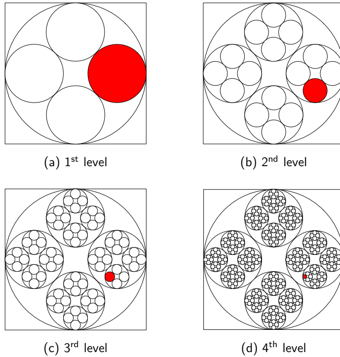
Figure 1: Illustration of the fractal decomposition of the search space: the depth of the decomposition is equal to 4.
