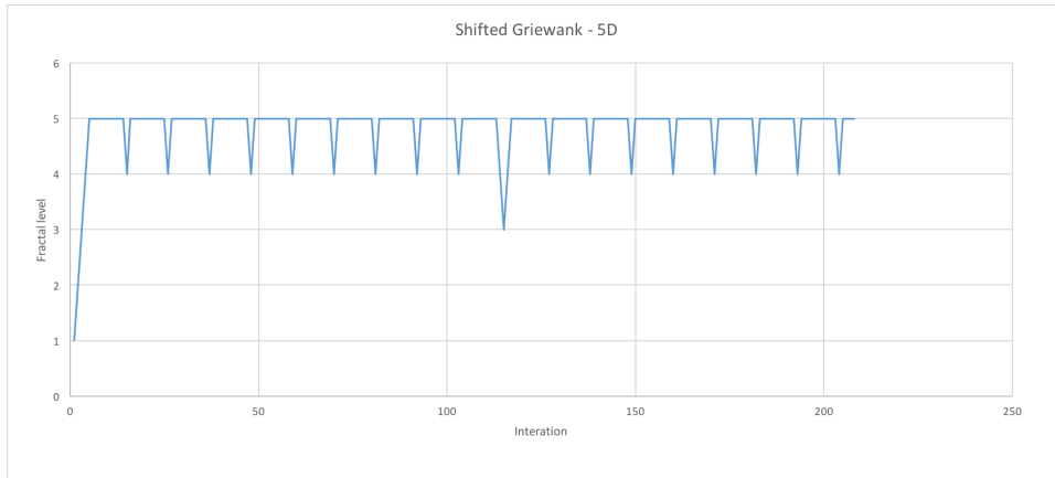
Figure 3: Illustration of the way FDA backtracks in the search tree in dimension D = 5
