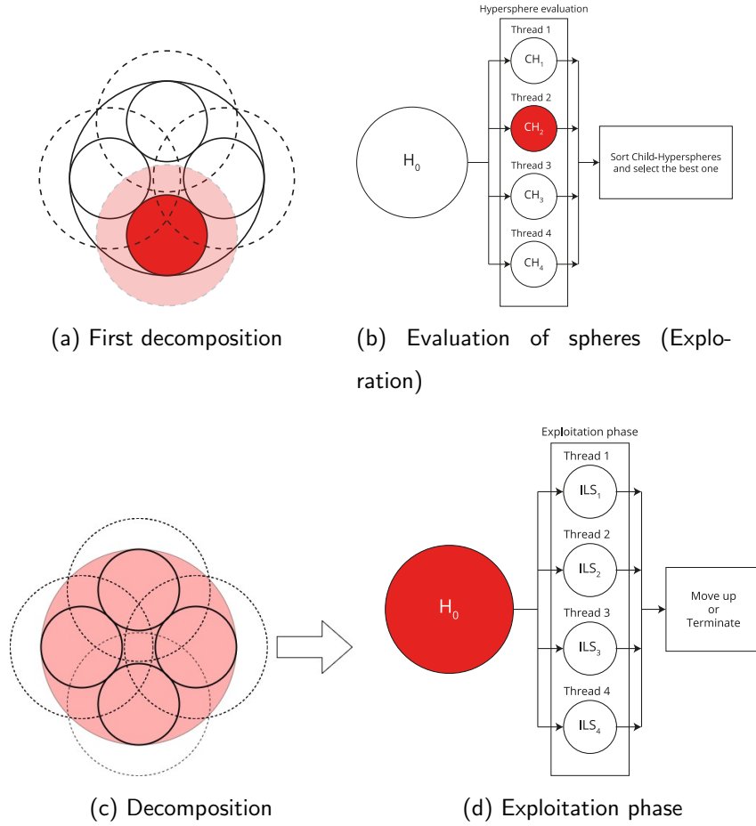
Figure 6: Illustration of the proposed strategy. Illustration of Exploration phase (a) and (b) and the Exploitation phase (c) and (d) of a 2D problem with fractal depth 2 on a multi-threaded environment. The child-hypersphere in red having the highest quality at level 1 (a) is being decomposed (c) for exploitation phase (d) which is also ran on a multi-threaded environment
