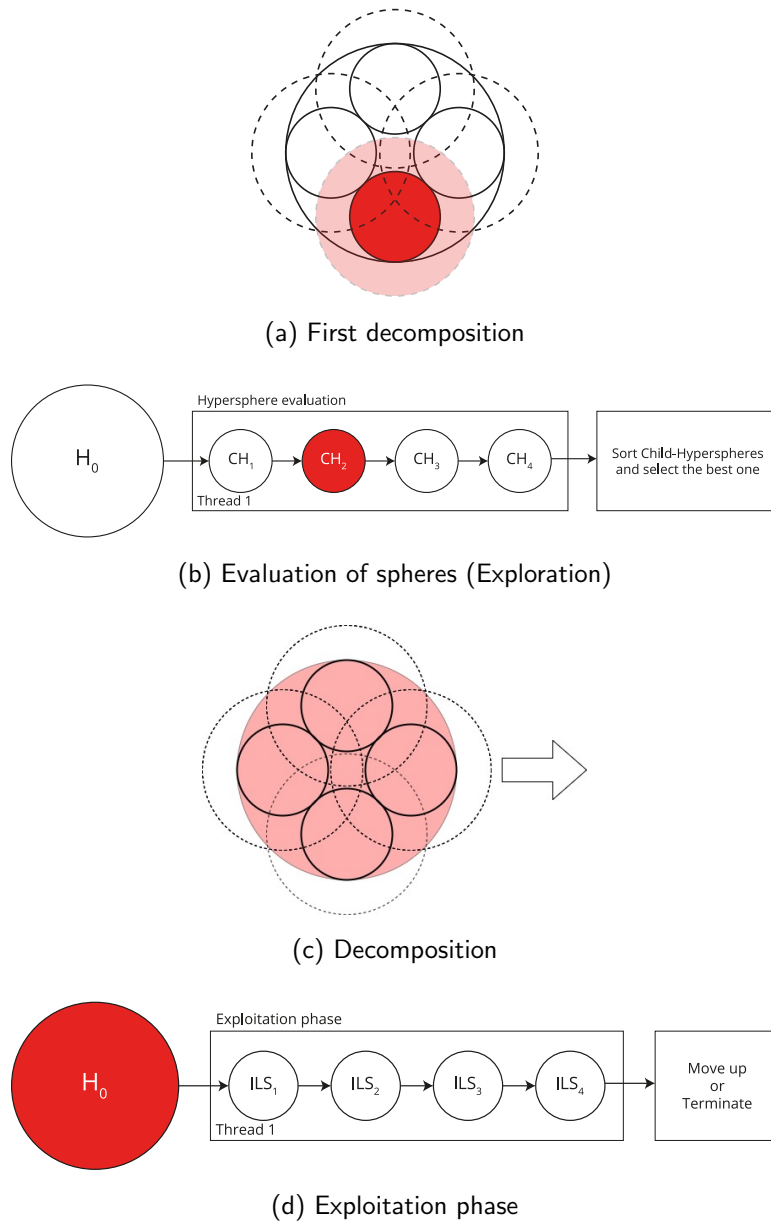
Figure 5: Illustration of Exploration phase (a) and (b) and the Exploitation phase (c) and (d) of a 2D problem with fractal depth 2 on a single threaded environment. The sphere in red having the highest quality at level 1 (a) and being decomposed (c) for exploitation phase (d).
