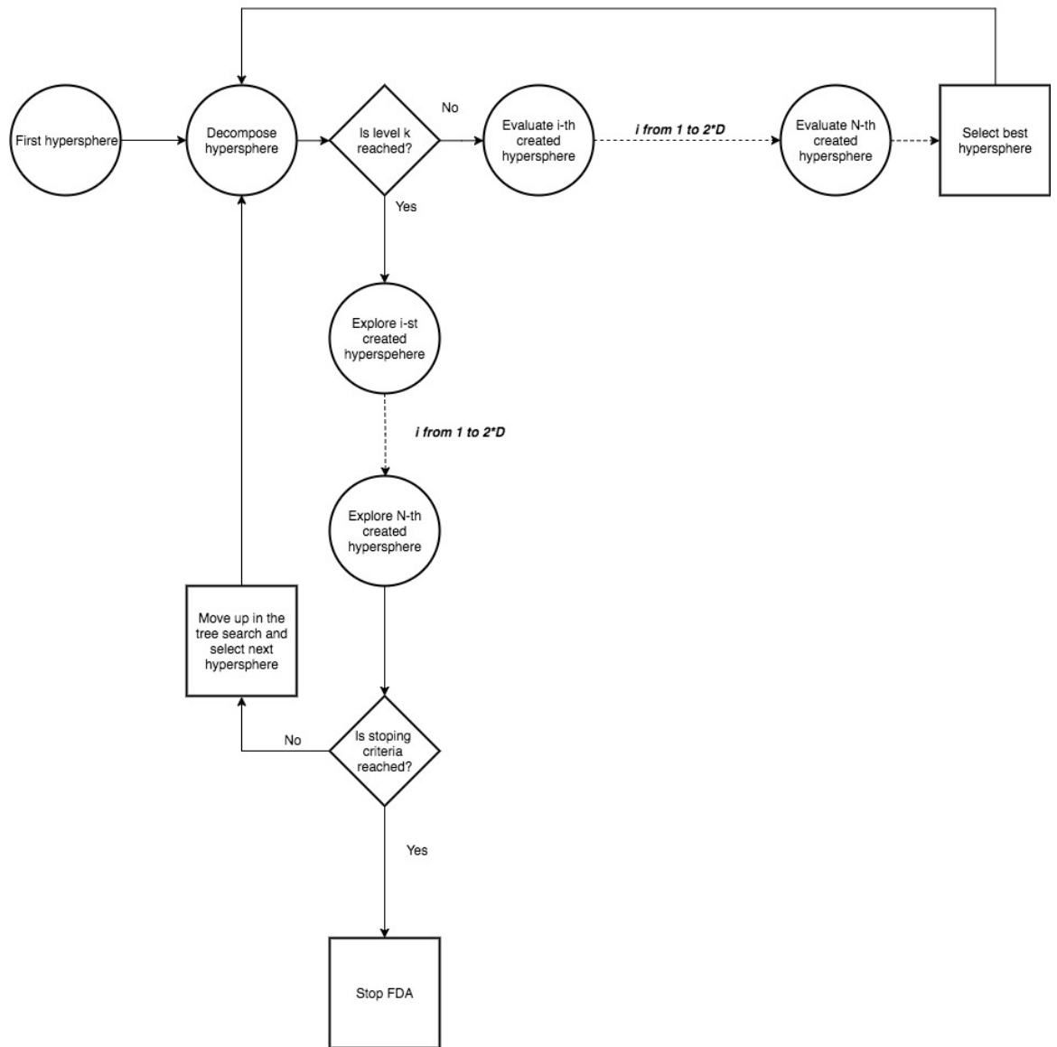
Figure 4: Illustration of life-cycle of the mono-threaded version of FDA.
