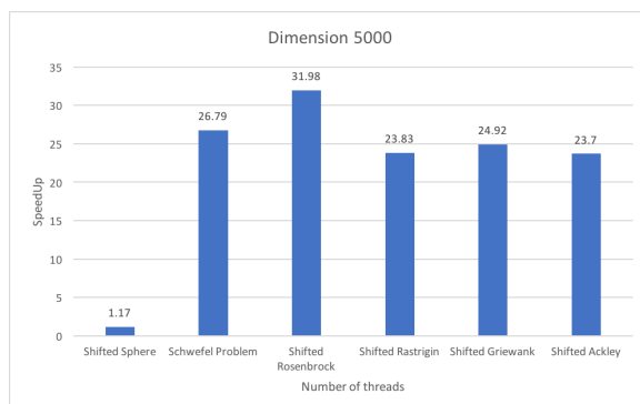
Figure 11: SpeedUp at dimension D = 5000 for the first six functions of the benchmark SOCO 2011 with number of threads n = 64
