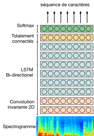
FIGURE 1 – Architecture neuronale DeepSpeech 2
