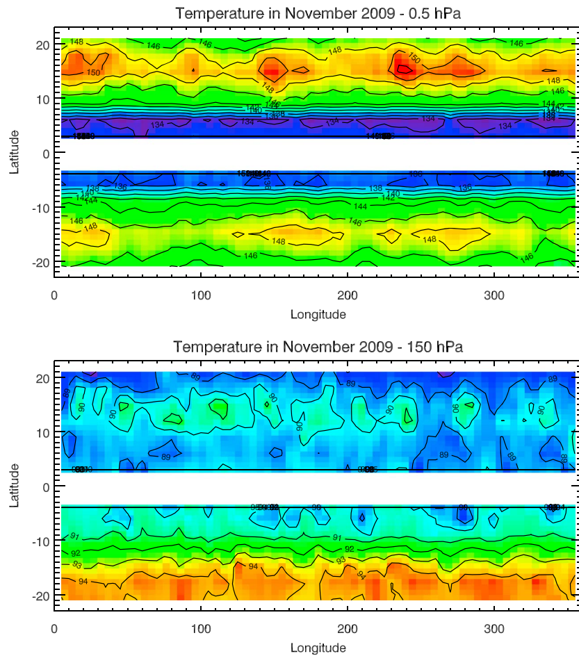
Figure 6. Maps of the temperature at (top) 0.5 hPa and (bottom) 150 hPa (retrieved from a Cassini/CIRS FIRMAP in November 2009. At 0.5 hPa, thermal waves with a peak-to-peak amplitude of 2.5 K and wave number 3 are clearly visible at both 15°S and 15°N. Spectra were co-added in bins of 10° wide in longitude, with a step of 5°, and bins 4° wide in latitude, with a step of 3°. The equatorial region is missing as the rings were contaminating the spectra in this region.
