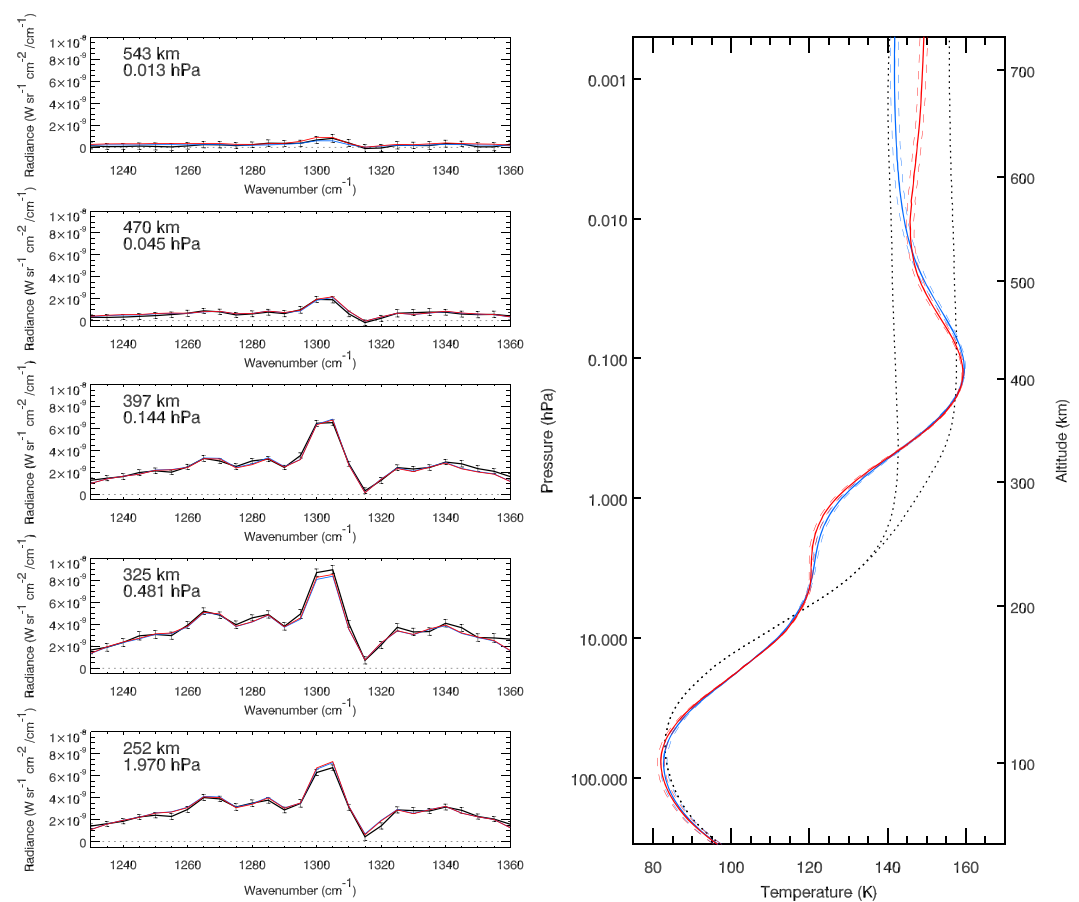
Figure 1. (left) Best fits (in red and blue, corresponding to different a priori profiles) to the \nu_4 methane band observed by Cassini CIRS in limb-viewing geometry at 2°N (in black, with 1 \sigma error bars). Spectra acquired at five different tangent altitudes are shown, which represent a subset of the eight spectra analyzed in total. Tangent altitudes and corresponding pressure levels are given in the upper left of each panel. (right) Corresponding retrieved profiles, in red and blue, starting from two different a priori profiles (black dotted lines). Above a certain level (here 0.01 hPa), the information content is poor and the temperature returns to the prior profile. In this example, we cannot discriminate between the two solutions (in blue and red) since the fits to the spectra are similar.
