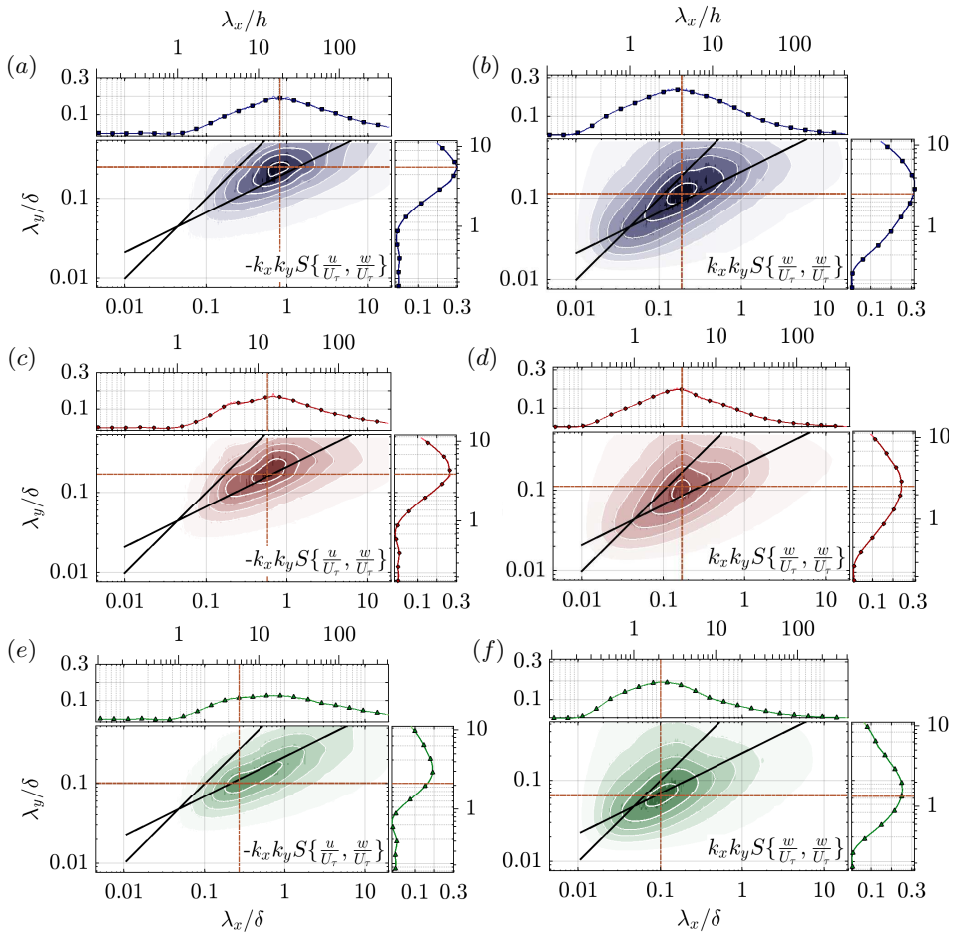
FIGURE 13. (Colour online) Pre-multiplied spectra in streamwise-spanwise plane z_1 = 1.5h for (a, b) \lambda_p = 6.25\% , (c, d) \lambda_p = 25\% and (e, f) \lambda_p = 44.4\% (see figure 11 for details). From left to right, (a, c, e) co-spectra -k_x k_y S\{u, w\} , and (b, d, f) auto-spectra k_x k_y S\{w, w\} .
