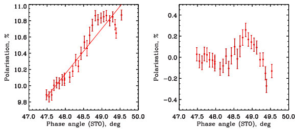
Figure 1. The phase angle (Sun–Target–Observer) dependence on the polarization is presented in the left-hand panel of the figure. The points represent the SDSS r' filter measurement from Rozhen with 1\sigma error bars. The solid line is the linear least-squares fit to the data, which is the behaviour we expect for this range of phase angles. The right-hand panel represents the polarization residuals after subtracting the best-fitting curve from the data.
