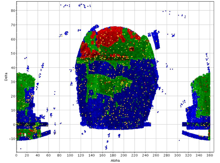
Fig. 14. Equatorial coordinates of the SDSS quasars plotted in Fig. 13. The colour codes of the quasars remain the same.
