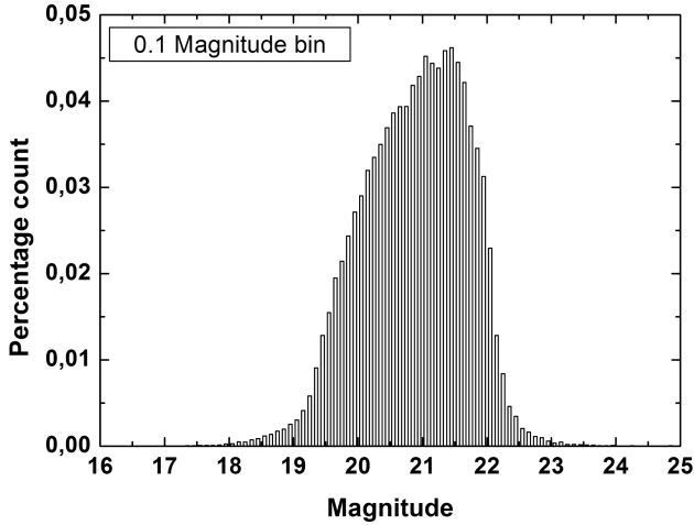
Fig. 17. Magnitude distribution histogram for the 121 461 new quasars in the LQAC4 for which DSS images and the morphological indexes were searched for and calculated. The percentage counts are obtained in 0.1 magnitude bins. The magnitudes are nearly all R, or otherwise in the closer optical band available. The average magnitude is 20.86, and the mode is 21.45, which values are as those of the LQAC3 version. No dependence of the morphological indexes with magnitude is found.
