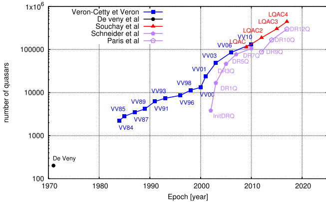
Fig. 1. Evolution of the number of objects in several quasar compiled catalogues: de Veny et al. (1971), the Véron-Cetty & Véron (2010) catalogue, and the Large Quasar Astrometric Catalogue. We also show one of the most ambitious surveys that bring a huge number of quasars to our knowledge: the Sloan Digital Sky Survey (York et al. 2000).
