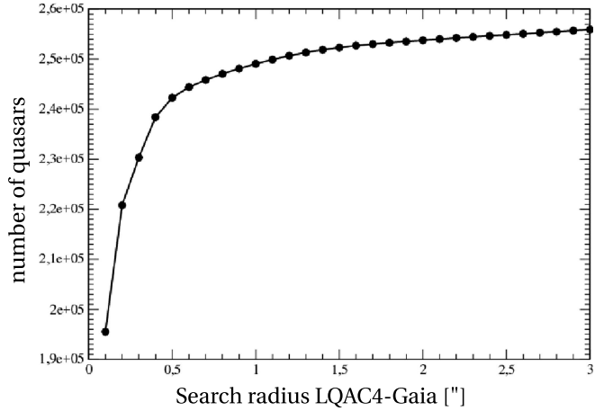
Fig. 6. Number of cross-matches between the LQAC-4 and the Gaia DR1, as a function of the search radius.
