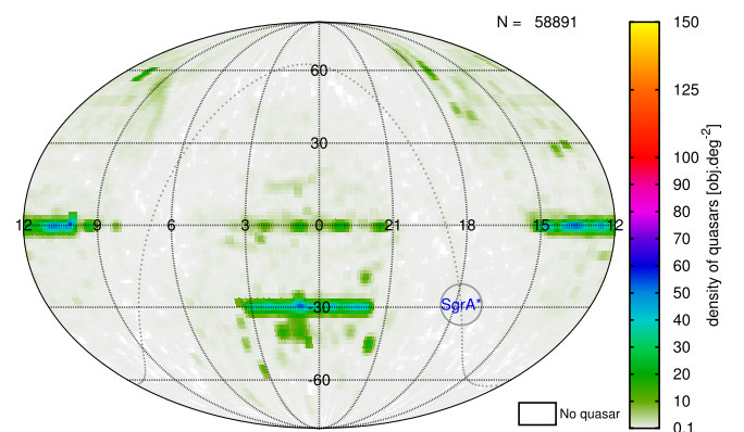
Fig. 5. Celestial sphere of the density map of quasars in the LQAC-4 but not in SDSS in equatorial coordinates. The curved dotted line represents the galactic plane. SgrA* indicates the centre of our galaxy.
