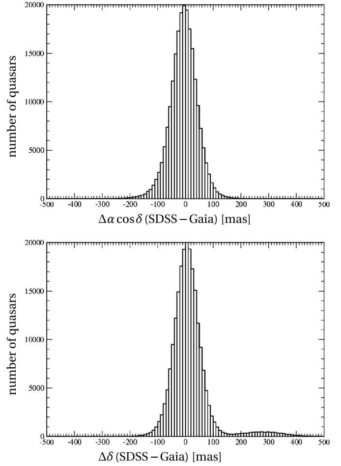
Fig. 11. Distribution of the differences in right ascension ( top ) and in declination ( bottom ) between the SDSS and the Gaia positions, limited to the quasars with values within \pm 500 mas.
