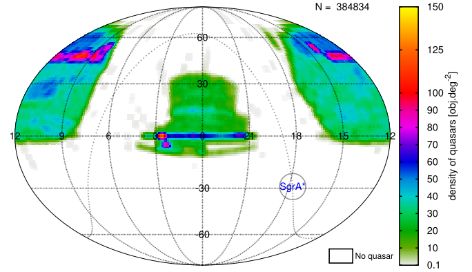
Fig. 4. Celestial sphere of the density map of quasars in the SDSS in equatorial coordinates. The curved dotted line represents the galactic plane. SgrA* indicates the centre of our galaxy.
