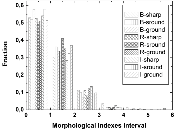
Fig. 19. Histograms of the morphological indexes for the new quasars in the LQAC4. The binsize in abscissa is reduced for the sake of clarity. Each bin refers to the integer range in which it is located (e.g. [0, 1]). The fractions in ordinate refers to the total number of sources for which each of the nine morphological indexes were determined. Letters B , R , and I refer to the three colours of DSS plates, blue, red, and infrared. The mnemonic after the letters refer to the IRAFA’s DAOFIND morphological index, respectively sharp, sround, and ground.
