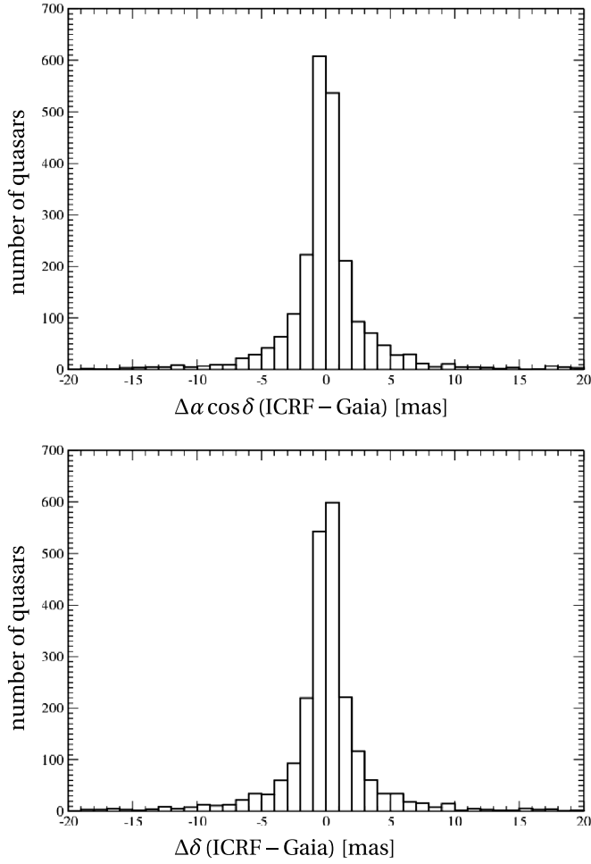
Fig. 9. Distribution of the differences in right ascension ( top ) and in declination ( bottom ) between the ICRF2 and the Gaia positions, for the quasars with values within \pm 20 mas.
