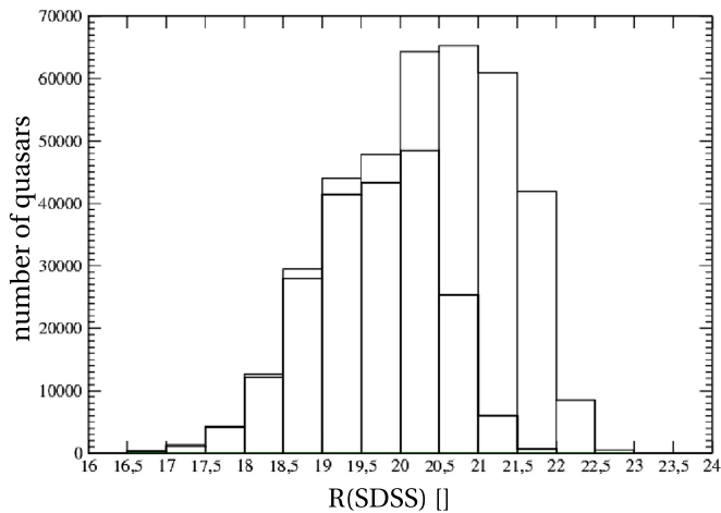
Fig. 8. Histogram of the number of SDSS quasars per bin of r (SDSS). In bold we plot the number of quasars reckoned by cross identification with Gaia -DR1.
