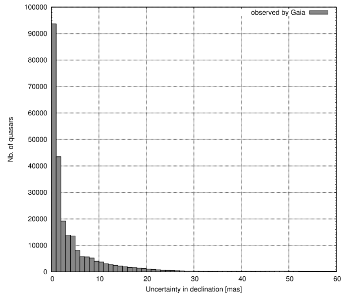
Fig. 21. Histogram of uncertainty in declination of the 249 071 quasars of the LQAC-4 cross-matched with Gaia . Values are taken directly from the Gaia DR1
