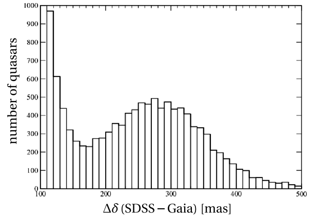
Fig. 12. Distribution of the differences in declination between the SDSS and the Gaia positions, limited to the quasars with values between 100 mas and 500 mas.
