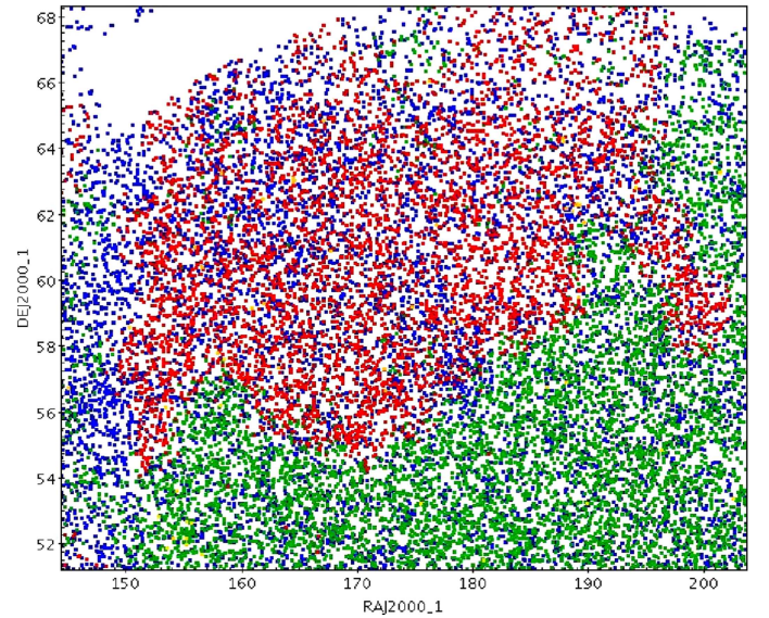
Fig. 15. Magnification of Fig. 14 above.
