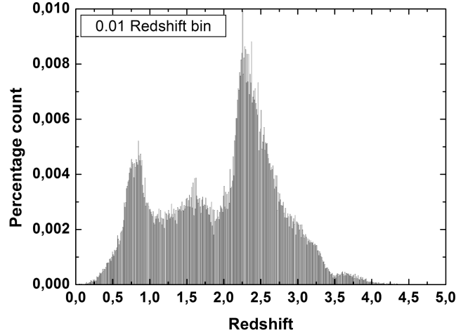
Fig. 18. Redshift distribution histogram for the 121 461 new quasars in the LQAC4 for which DSS images and the morphological indexes were searched for and calculated. The percentage counts are obtained in 0.01 redshift bins. All redshift are spectroscopic. There are clearly two concentrations, inherited from the SDSS Main and BOSS populations.
