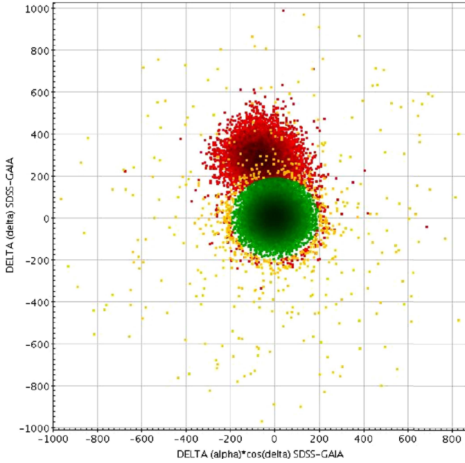
Fig. 13. Two-dimensional plot of the offsets \Delta\delta vs. \Delta\alpha \cos\delta of the SDSS with respect to the Gaia DR1 positions. In blue we plot the SDSS quasars for which \rho < 200 mas, belonging to the LQAC-3; in green, the SDSS quasars for which \rho < 200 mas, belonging to the DR12Q (LQAC-4–LQAC-3); in yellow, the quasars with \rho > 200 mas belonging to the LQAC-3; in red, the SDSS quasars with \rho > 200 mas belonging to the DR12Q (LQAC-4–LQAC-3).
