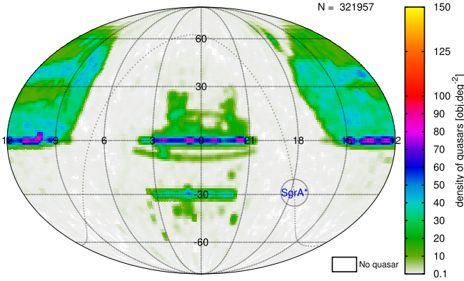
Fig. 2. Celestial sphere of the density map of quasars in the LQAC-3 in equatorial coordinates. The curved dotted line represents the galactic plane. SgrA* indicates the centre of our galaxy.
