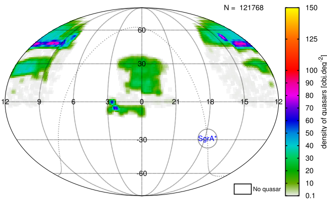
Fig. 3. Celestial sphere of the density map of new quasars (with respect to LQAC-3) in the LQAC-4 in equatorial coordinates. The curved dotted line represents the galactic plane. SgrA* indicates the centre of our galaxy.
