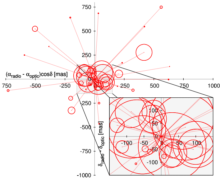
Fig. 10. Two-dimensional plot \Delta\delta vs. \Delta\alpha \cos\delta of the differences between the VLBI radio positions ICRF2 and the optical Gaia positions for the quasars with angular offset larger than 50 mas. Circles stand for the combined error of the two measurements.
