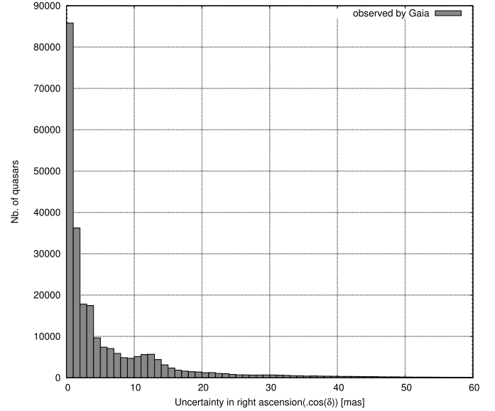
Fig. 20. Histogram of uncertainty in right ascension of the 249 071 quasars of the LQAC-4 cross-matched with Gaia . Values are taken directly from the Gaia DR1
