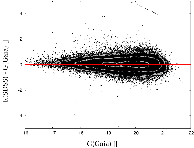
Fig. 7. Magnitude difference r (SDSS)- G ( Gaia ) for the quasars in common in the two surveys. Contour-plots are added to estimate the number of points in the saturated area. The largest, intermediate, and shortest contour-plots correspond respectively to, ten points, 50 points, and 250 points in a pixel of 0.05 magnitude \times 0.05 magnitude.
