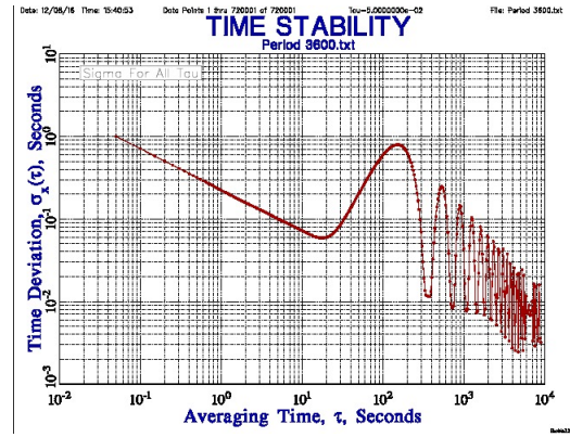
Fig. A.2. TDEV of a white-phase noise affected by a periodic signal of period T_0 = 360 s. The maxima are visible for averaging times \tau = \frac{T_0}{2}, \frac{3T_0}{2}, \frac{5T_0}{2}, \dots
