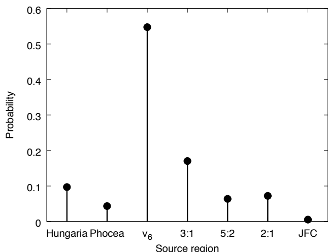
Fig. 2. Source regions of the 15 selected NEA that fulfil the criteria in spectral class and albedo range. The region with the highest probability on average is the v_6 , indicating that the source should be the inner main belt.
