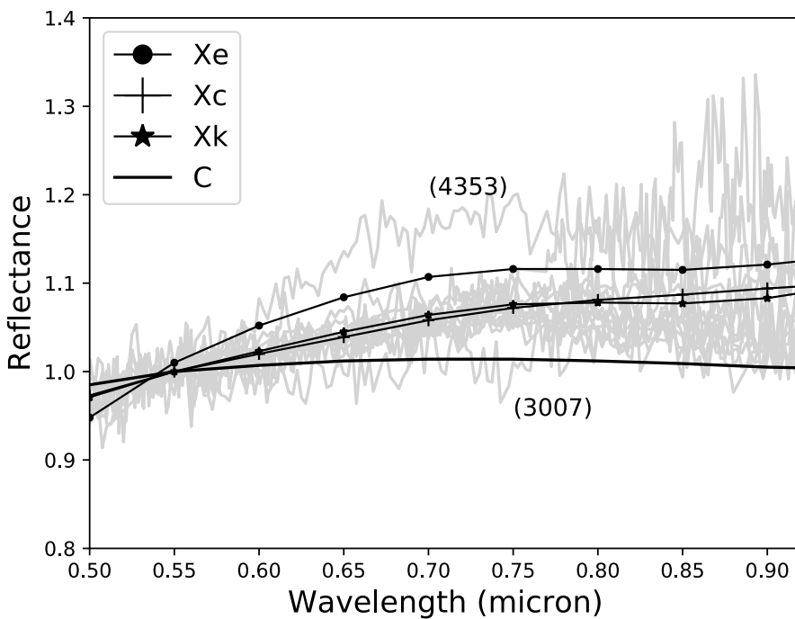
Fig. A.3. Reflectance spectra from the literature of Athor family members numbered 161, 757, 1697, 1998, 2194, 3007, 3665, 3704, 3865, 4353, 4548, 4839, and 4845. The average reflectance spectra of the Xe, Xc, Xk, and C of the DeMeo et al. (2009) taxonomy (from http://smass.mit.edu/_documents/busdemeo-meanspectra.xlsx ) are also plotted. References are: (161) from Bus & Binzel (2002), (757) from Bus & Binzel (2002), 1697 from Xu et al. (1995), (1998) from Bus & Binzel (2002), (2194) from Bus & Binzel (2002), (3007) from Bus & Binzel (2002), 3665 from Xu et al. (1995), (3704) from Bus & Binzel (2002), (3865) from Bus & Binzel (2002), (4353) from Bus & Binzel (2002), (4548) from Bus & Binzel (2002), (4839) from Bus & Binzel (2002), (4845) from Bus & Binzel (2002).
