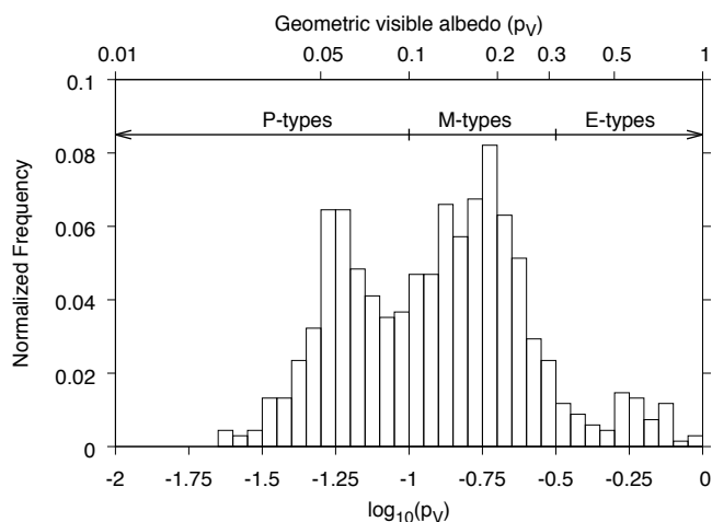
Fig. 1. Multimodal distribution of the geometric visible albedo of all asteroids belonging to the X complex (i.e. with spectral types found in literature being X, Xc, Xe, Xk, M, E, and P). The three peaks of the distribution correspond to the P-, M-, E-types of the Tholen & Barucci (1989) taxonomy, and their boundaries are defined p_V \leq 0.1 , 0.1 < p_V \leq 0.3 , and p_V > 0.3 , respectively, and are marked by the arrows at the top of the figure. As one can see these albedo boundaries provide reasonable separation between the classes. In this work we focus on X-complex asteroids with 0.1 < p_V \leq 0.3 , that is, the M-types of Tholen & Barucci (1989) , which in Bus-DeMeo mostly corresponds to the Xc-types.
