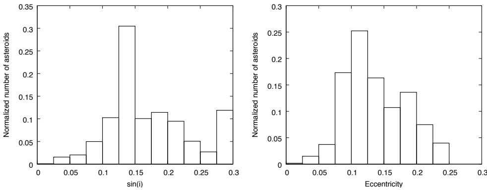
Fig. A.2. Distribution of the proper eccentricity and sinus of the proper inclination for X-type asteroids inside and near the border of the V shape with equation 1/D = 1.72 |a - 2.38| \text{ km}^{-1} (see text). The peaks show clustering of these asteroids, indicating the centre of the family.
