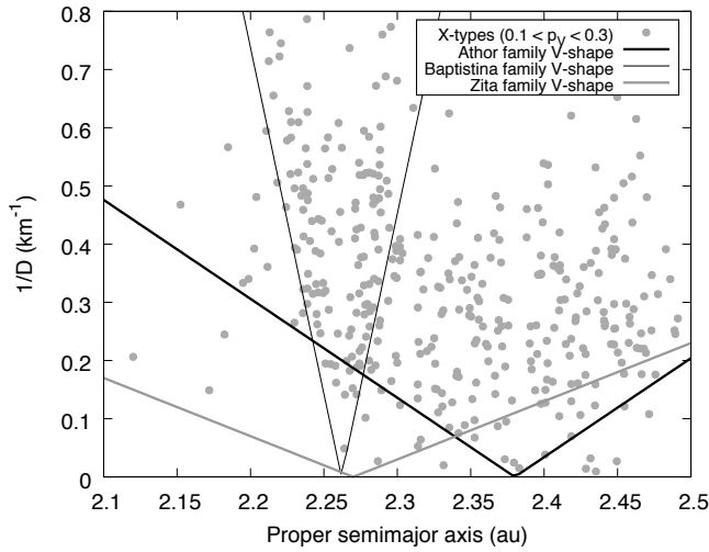
Fig. A.1. V shapes formed by the X-complex asteroids with geometric visible albedos in the range 0.1–0.3 of the inner main belt ( 2.1 < a < 2.5 au).
