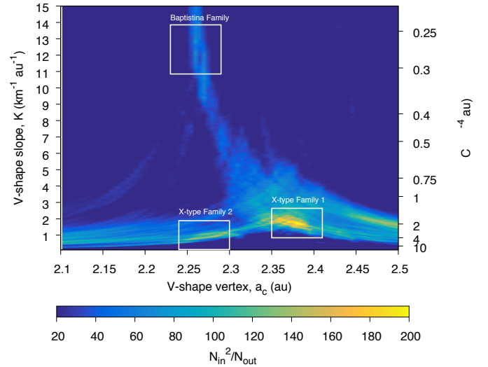
Fig. 3. Output of the V-shape-searching method. The value of N_{in}^2/N_{out} is plotted as a function of the slope ( K ) and semimajor axis of the vertex of a V shape ( a_c ). The value of the parameter C , which measures the width of a V shape in the (a, H) space, where H is the absolute magnitude (Vokrouhlický et al. 2006) and is calculated from C = 1/K \sqrt{p_V}/1329 using a geometrical visible albedo p_V = 0.2 .
