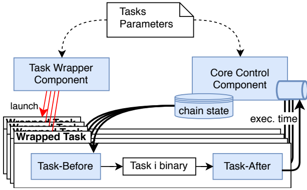
Fig. 1. Monitoring & Control Agent Architecture
