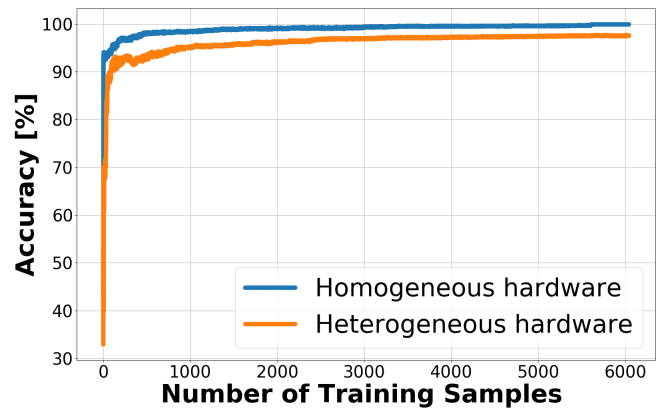
Figure 7. Learning curves on the testing set as a function of the number of training samples
