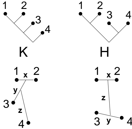
Fig. 2 Upper part: Tree diagram representing the two possible topological ways for breaking fully interacting 4-body cluster (1234) into substructures. Lower part: Jacobi coordinates corresponding to each cluster partition.
